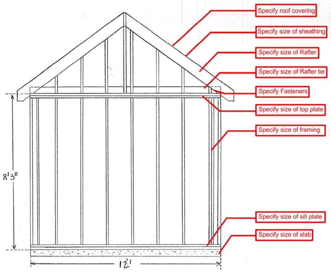
~ NORTH WALL FRAMING ~ SCALE 1/2" = ONE FOOT
