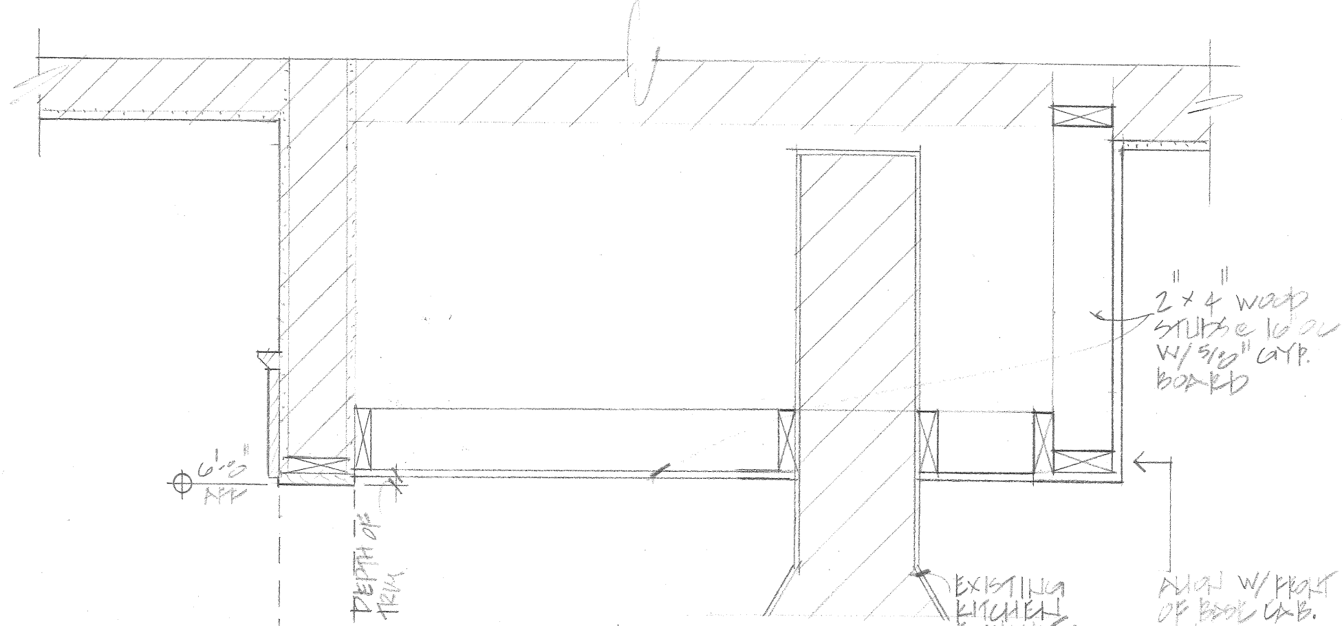
1 SECTION THROUGH SINKIT OVER RANGE/COUNTER EXISTING CAB SHOWN HATCHED
