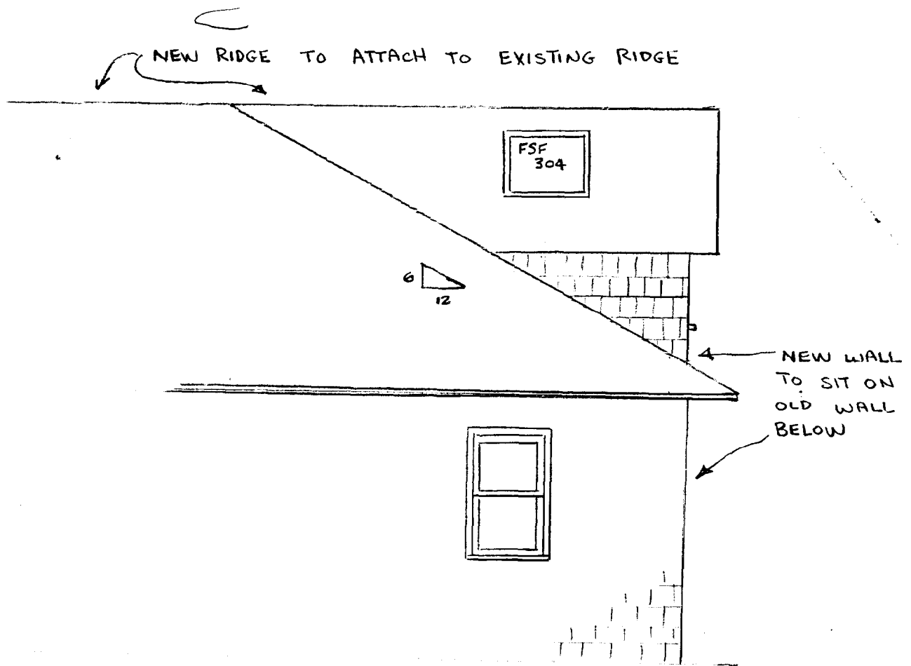
RIGHT SIDE (REAR) ELEVATION SCALE 1/4" = 1'-0"
