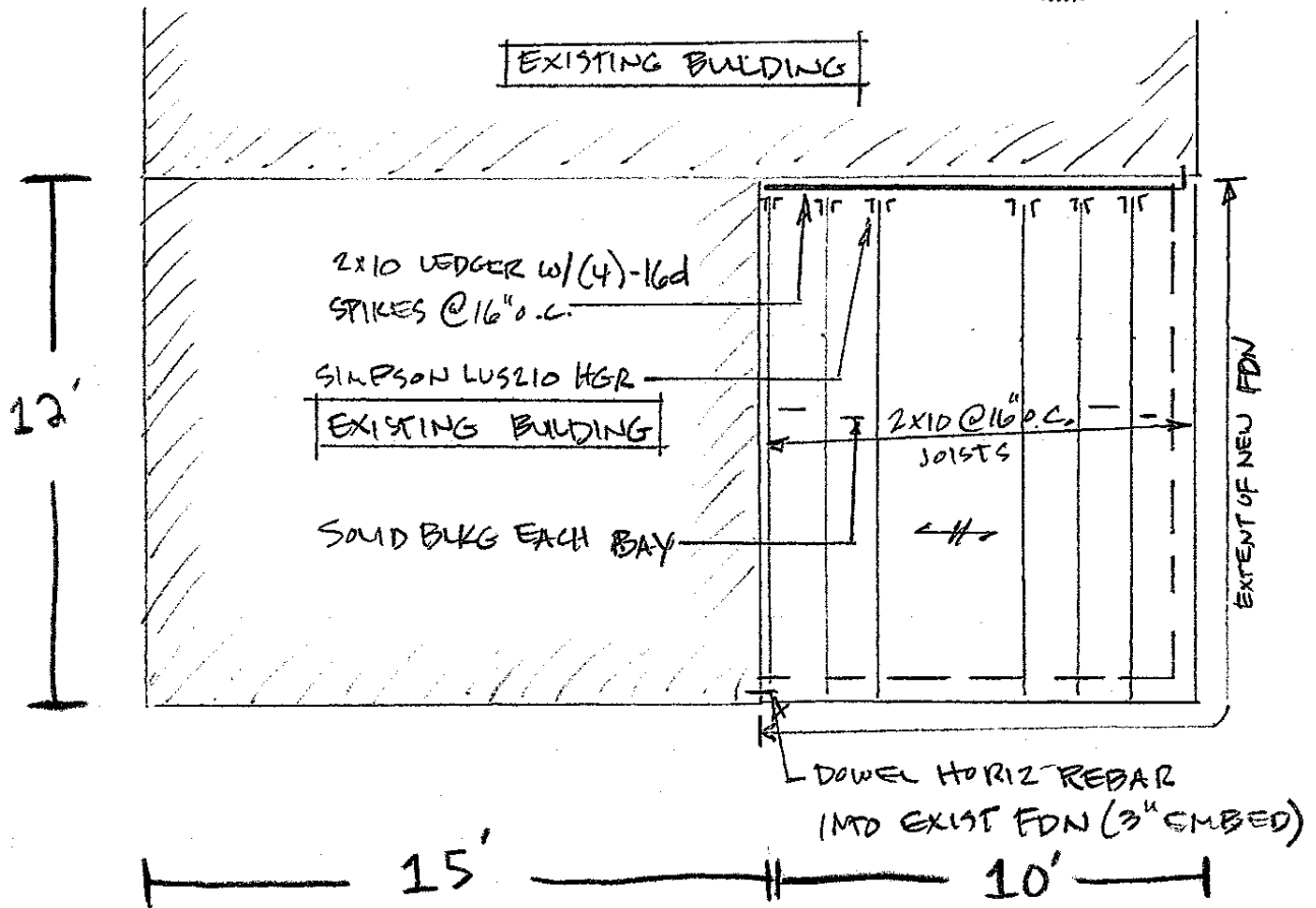
FOUNDATION / FIRST FLOOR FRAMING PLAN N.T.S.
