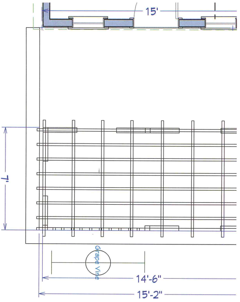
Trellis Plan 1/4 in = 1 ft
