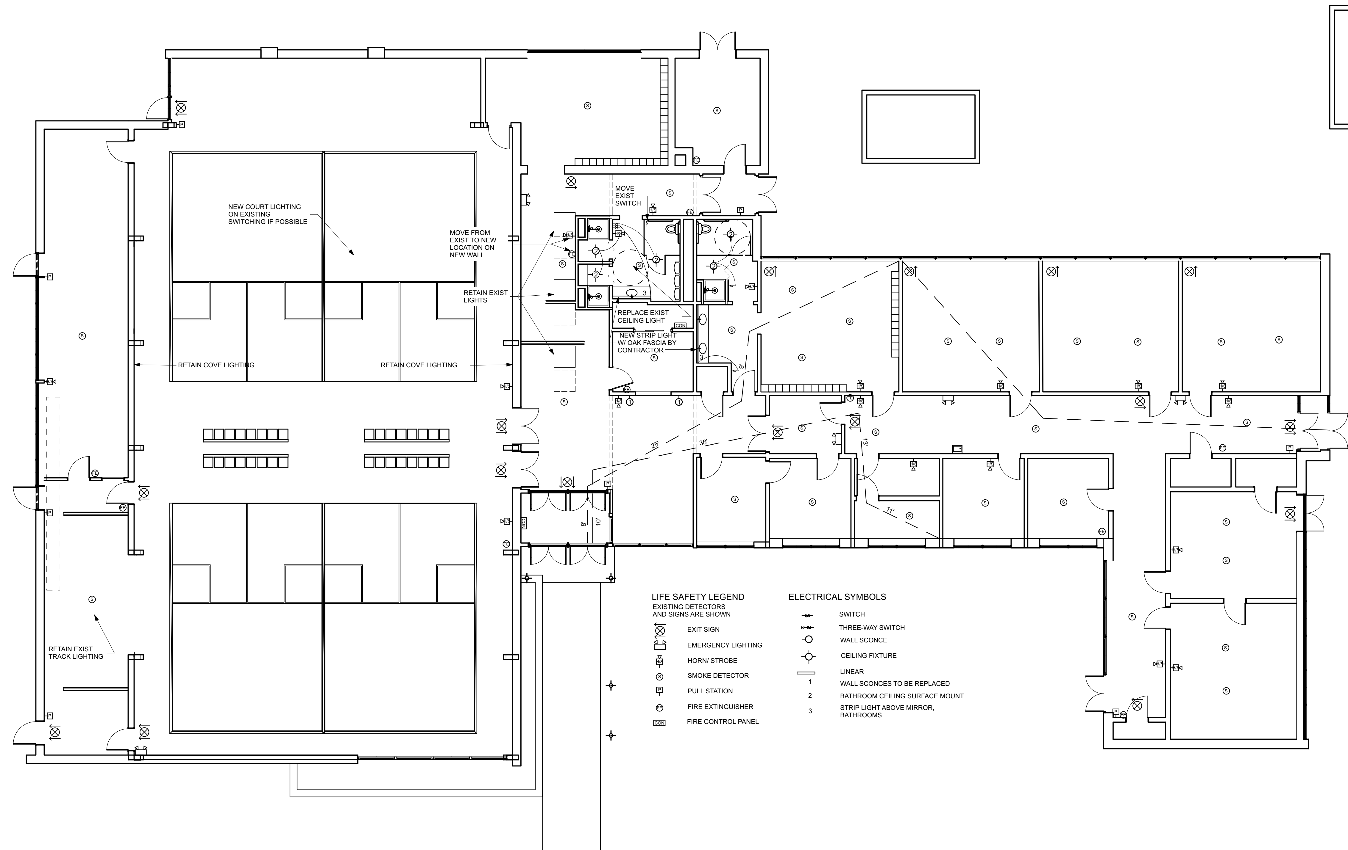
1 A-4.1 ELECTRICAL AND LIFE SAFETY PLAN SCALE: 1/8" = 1'-0"
