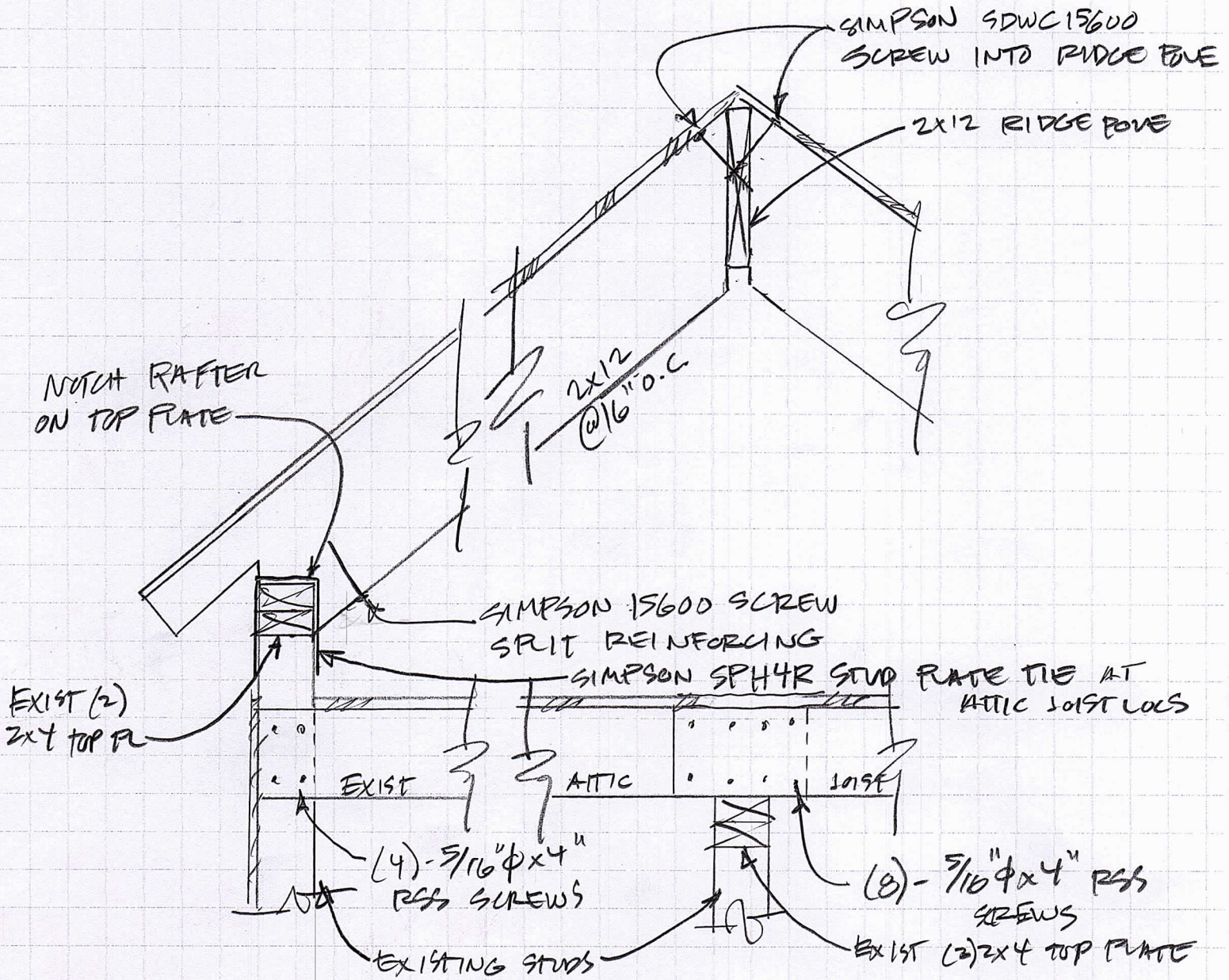
COLWAR TIE ROOF SECTION
