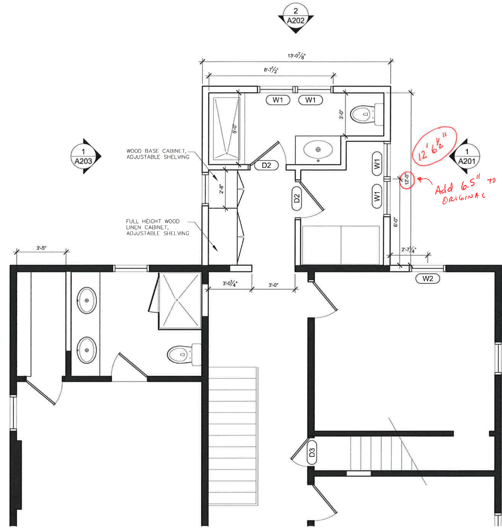
1 SECOND FLOOR PLAN SCALE: 1/4" = 1'-0"
