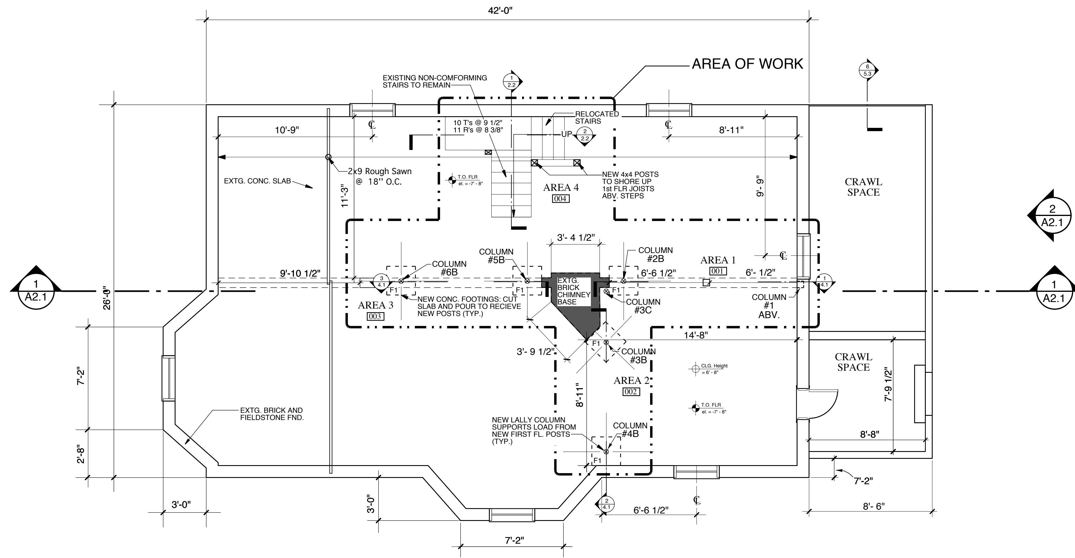
(A1.0) BASEMENT FLOOR PLAN SCALE: 1/4" = 1'-0"
