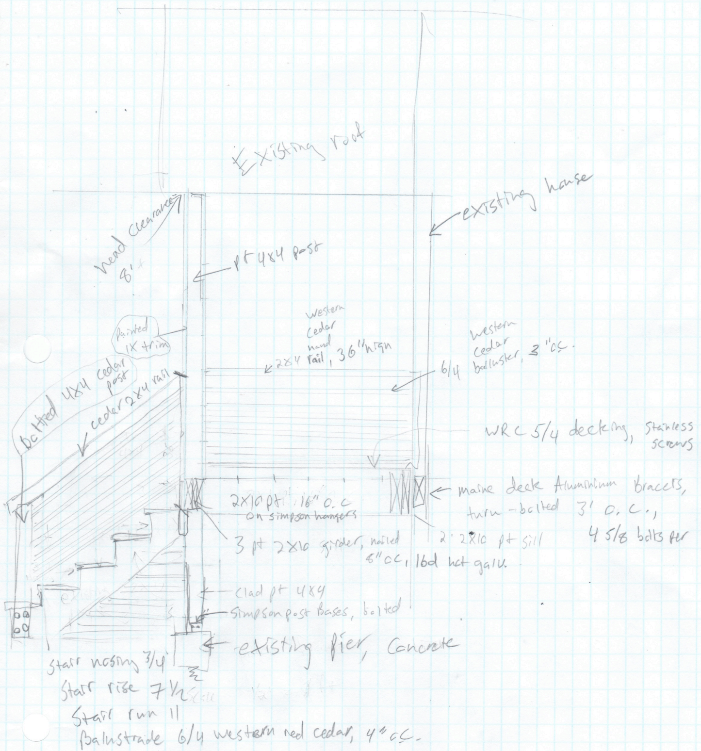
Porch Framing section Scale 1/2" = 1'
