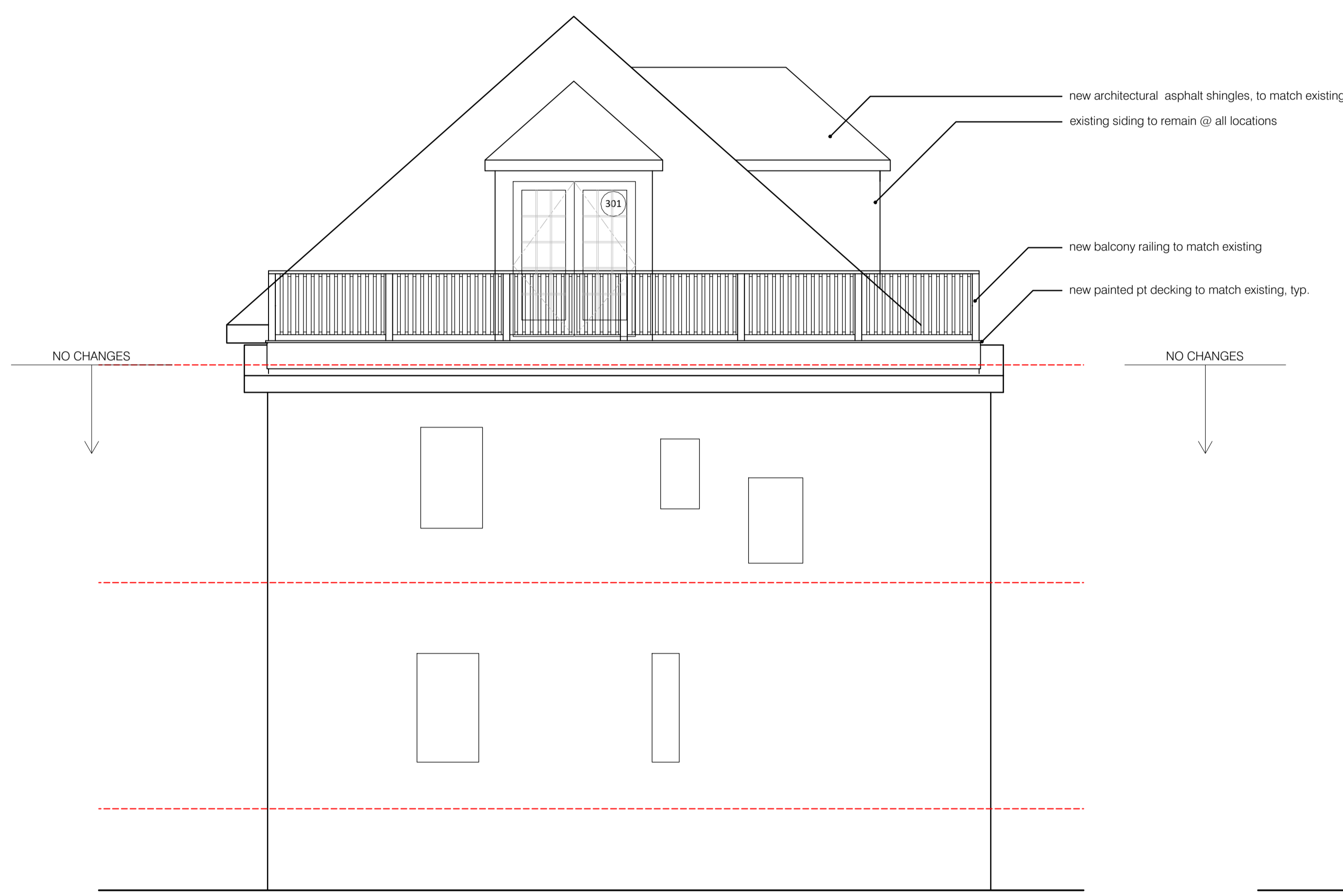
1 west elevation \frac{1}{4}'' = 1'-0''
