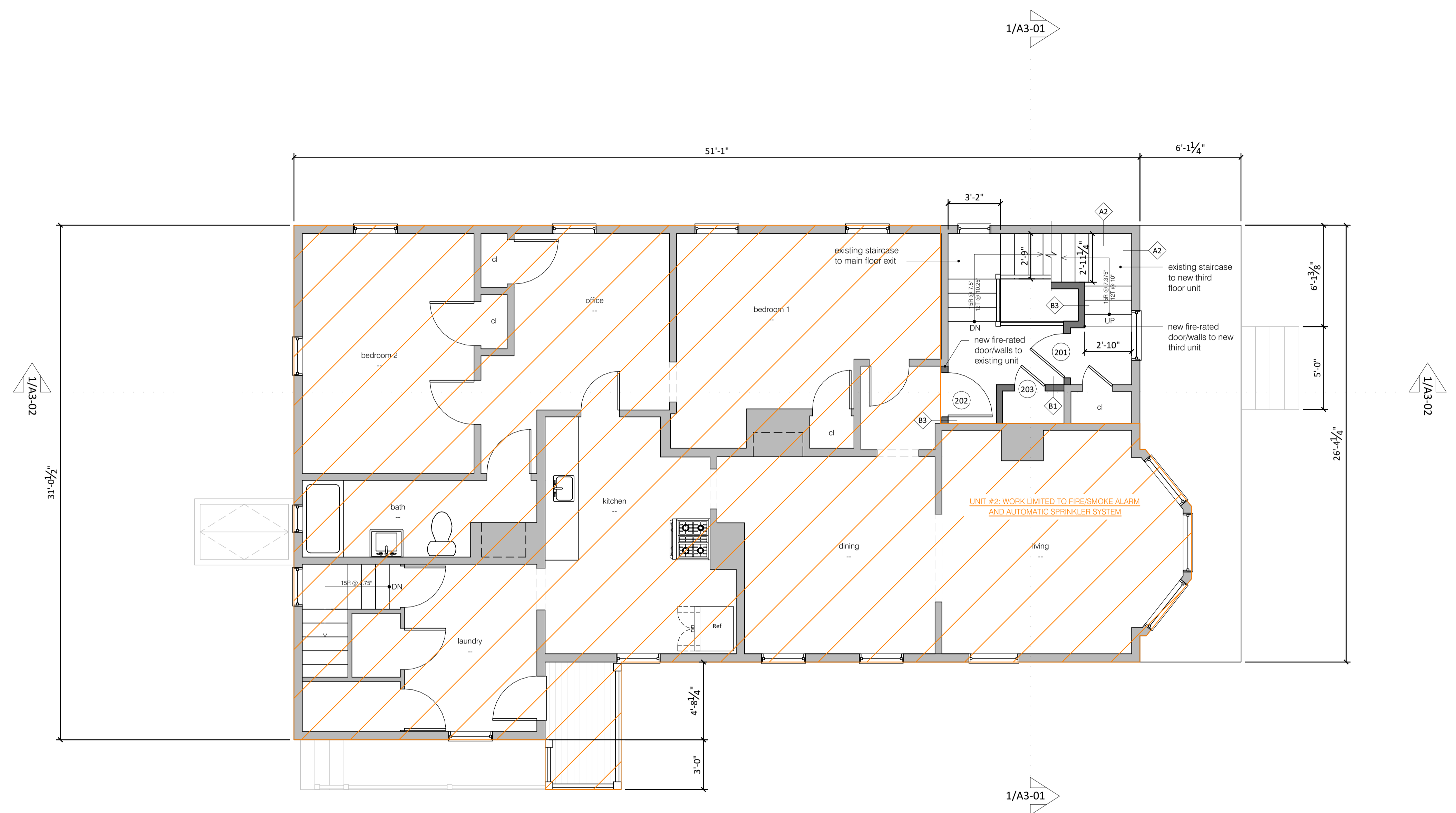
1 second floor plan 3/4" = 1'-0"
