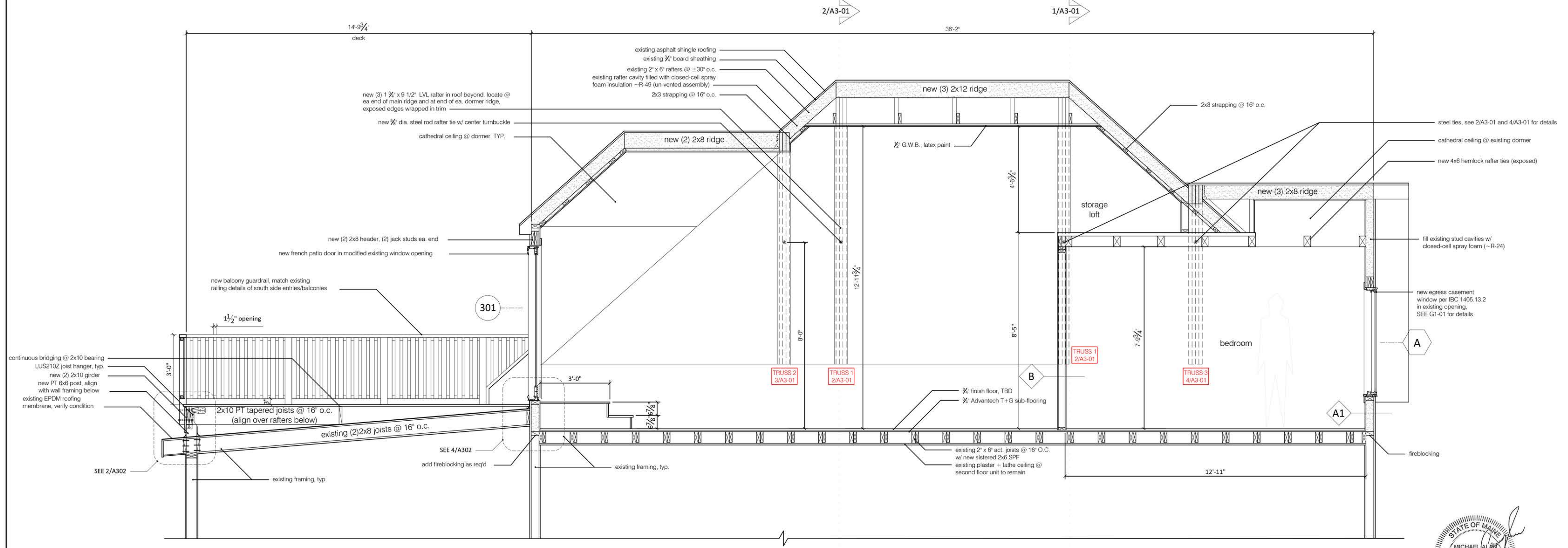
1 longitudinal building section 1/2" = 1'-0"
