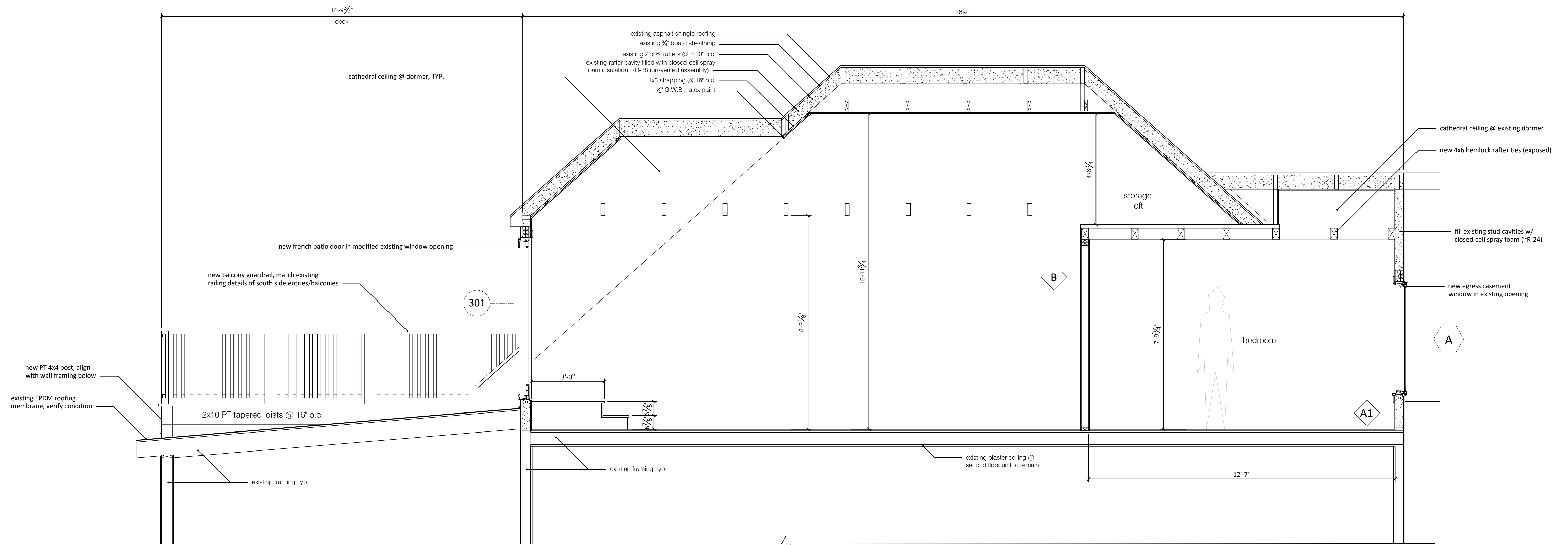
1 longitudinal building section 1/2" = 1'-0"
