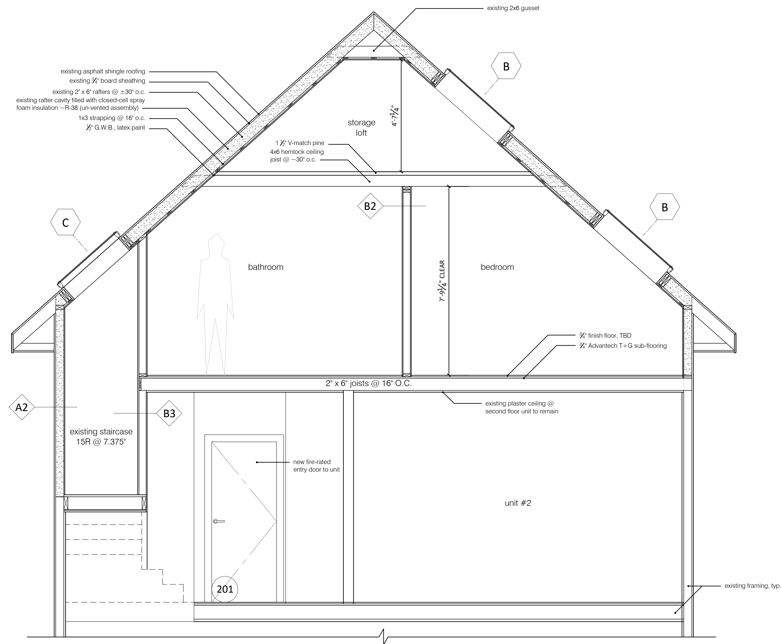
1 building section @ bedroom 1/2" = 1'-0"
