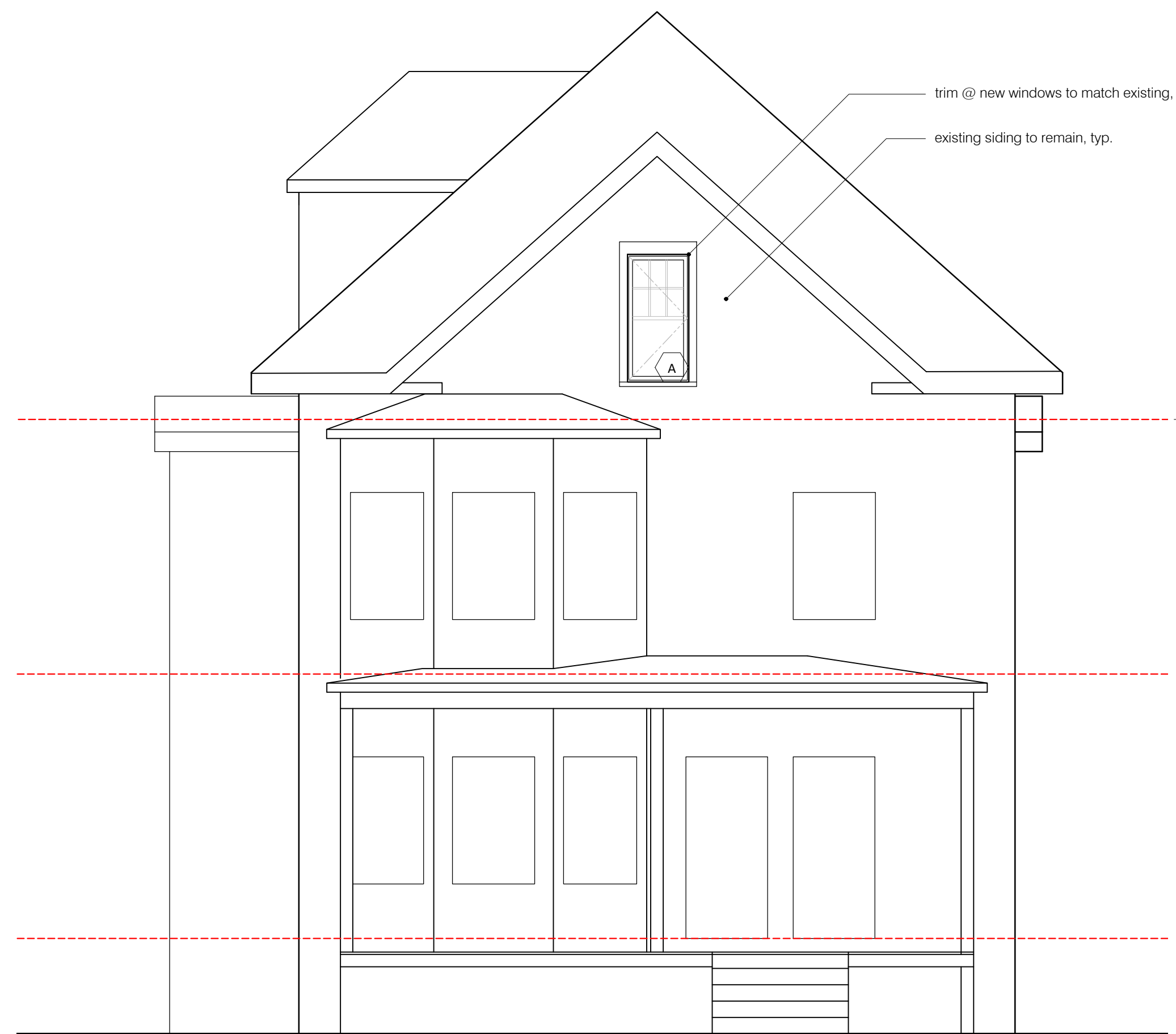
1 east elevation 1/4" = 1'-0"
