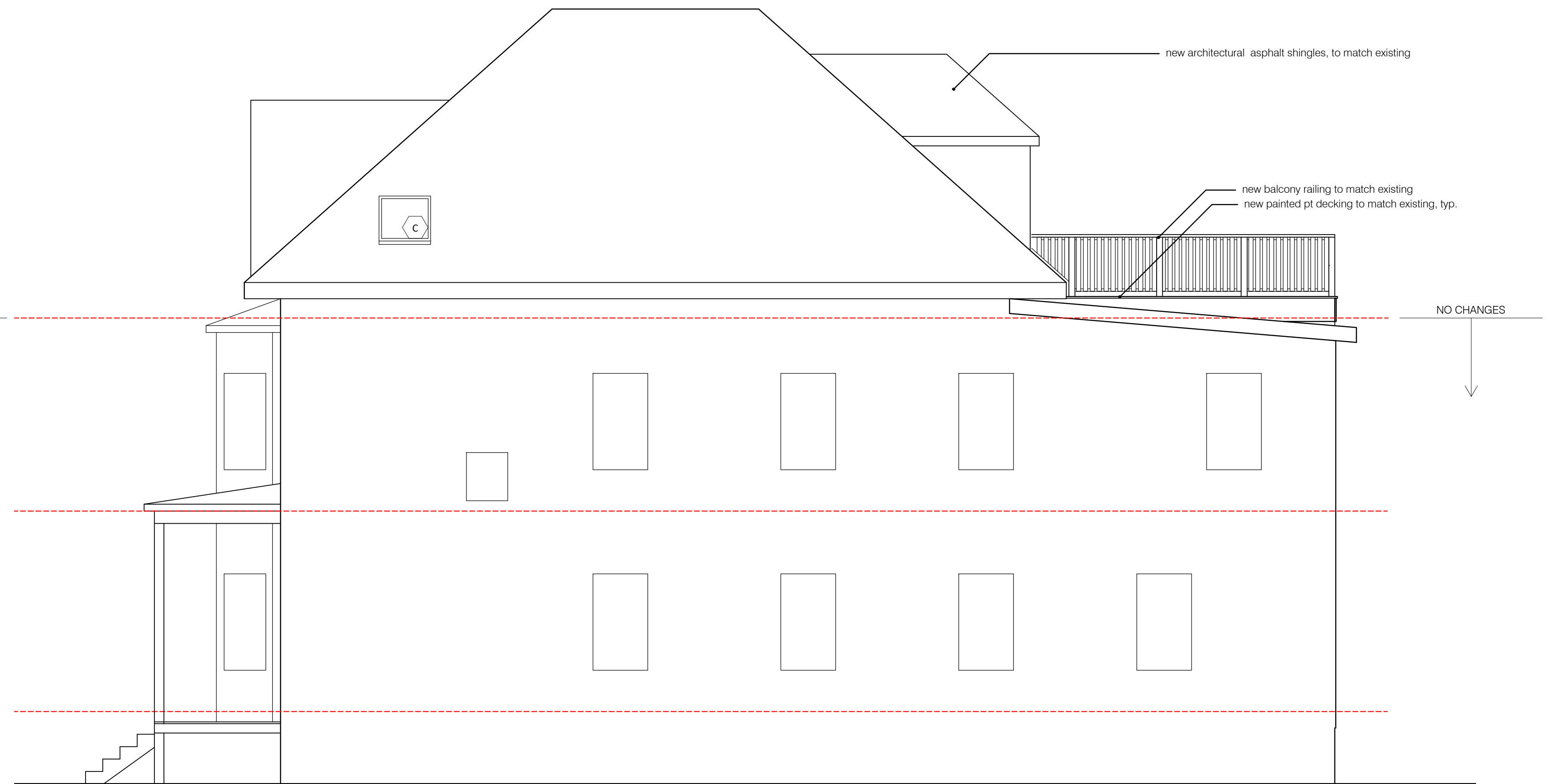
2 north elevation 1/4" = 1'-0"
