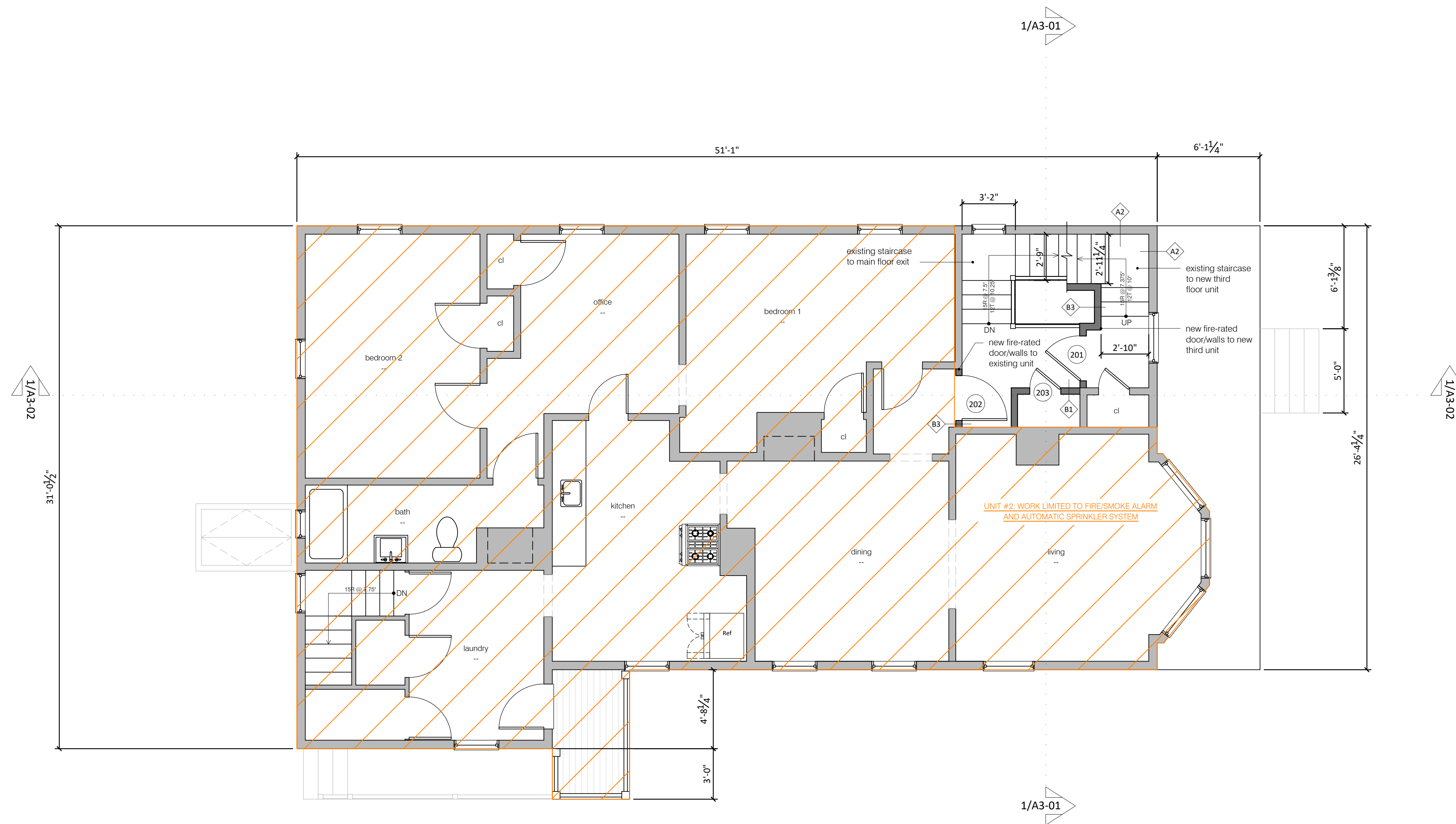
1 second floor plan 3/4" = 1'-0"
