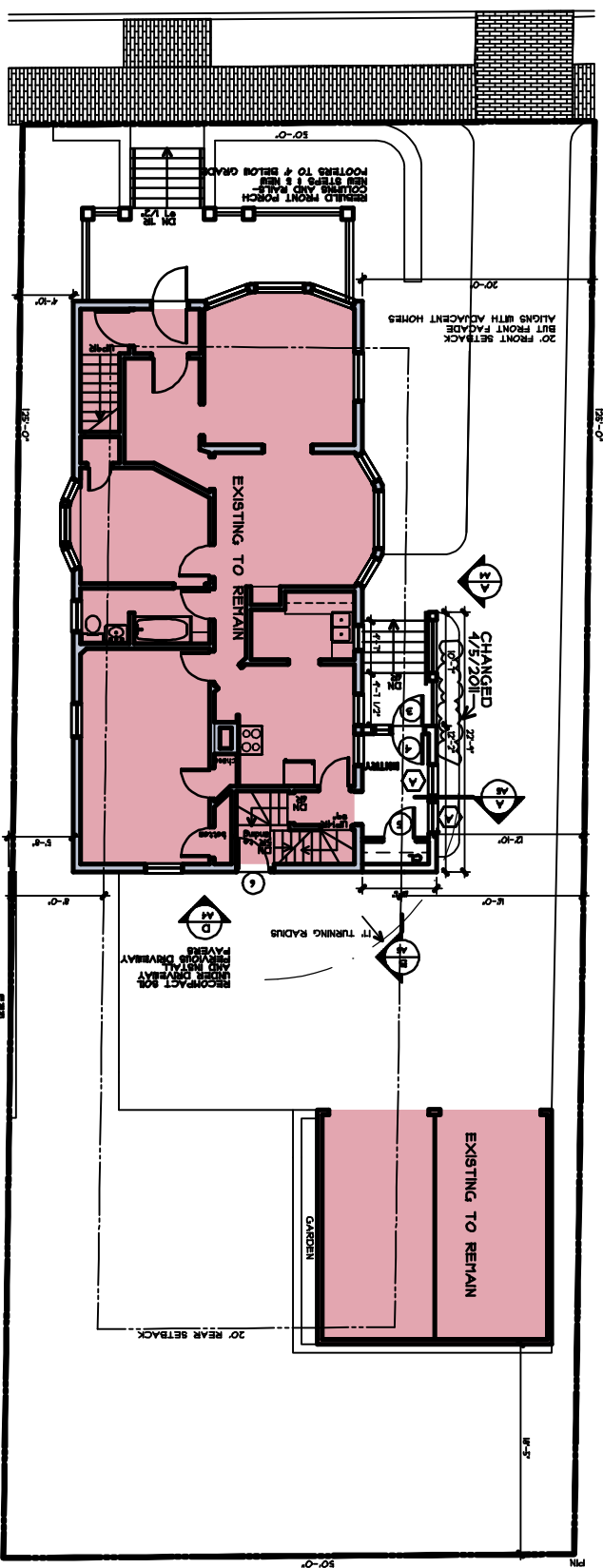
EXISTING SITE FIRST FLOOR PLAN 1/16" = 1'-0"
