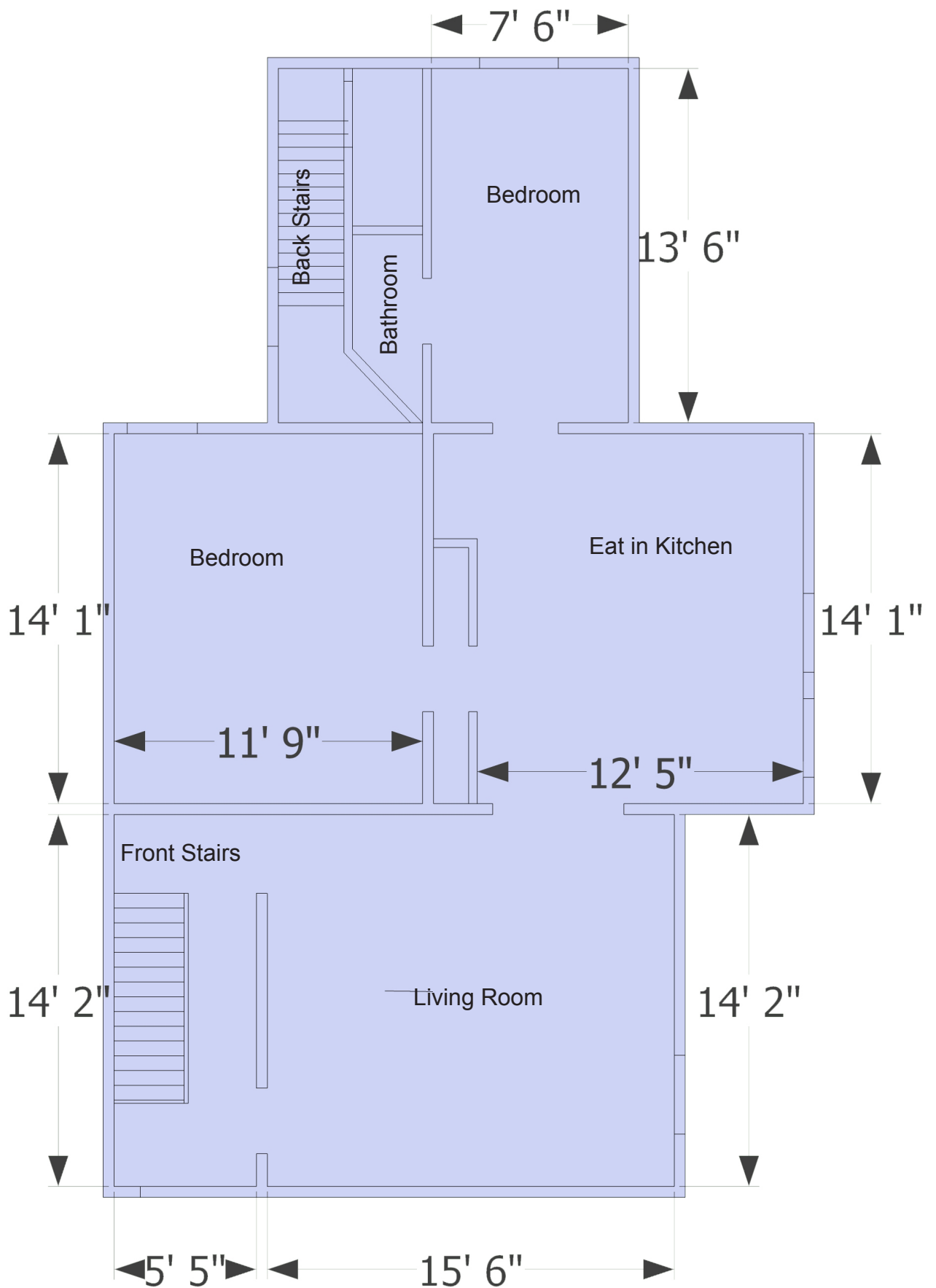
75 Fessenden Street 3rd Floor Plan. No Scale, see dims on plan. North is up.
