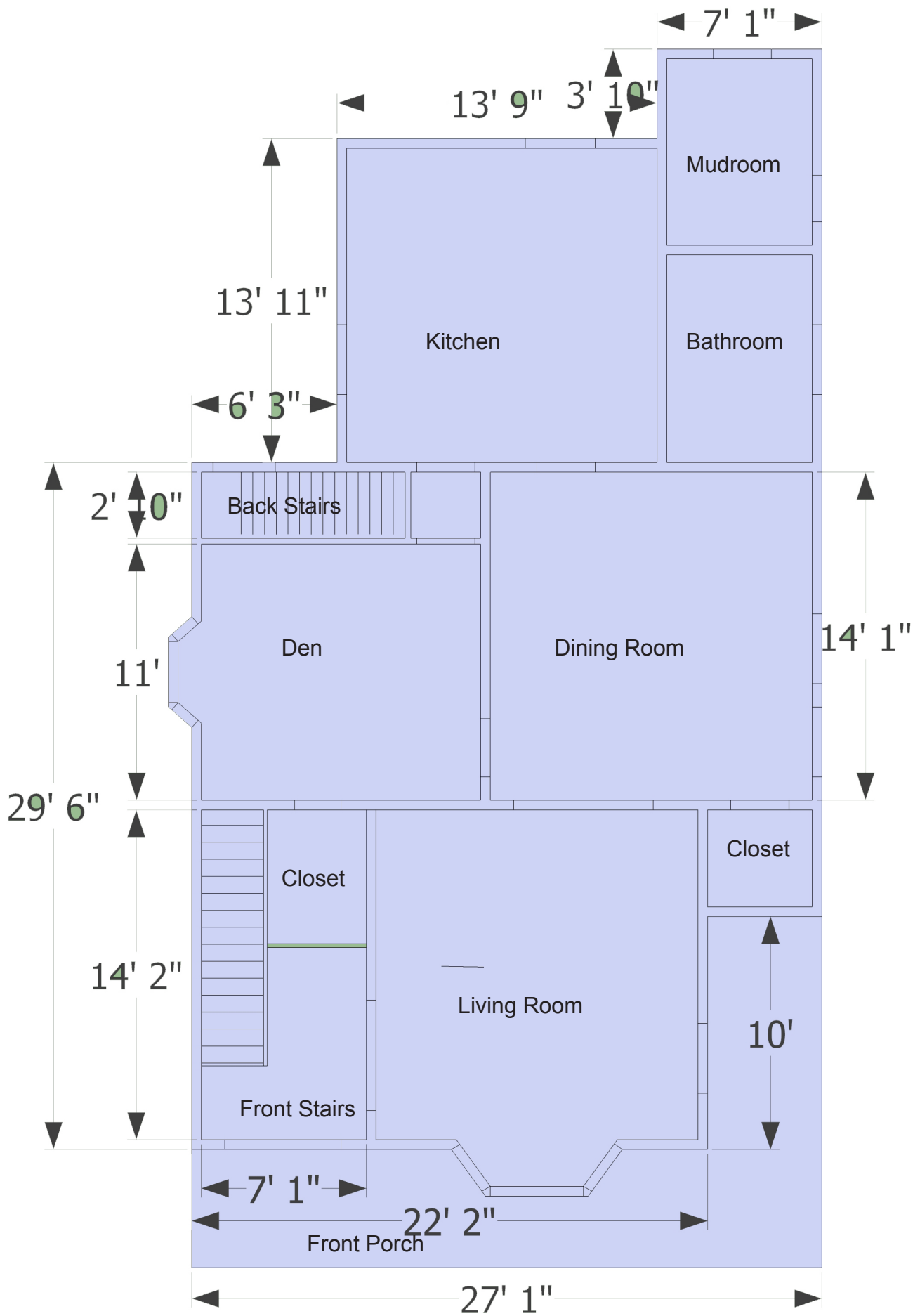
75 Fessenden Street 1st Floor Plan. No Scale, see dims on plan. North is up.
