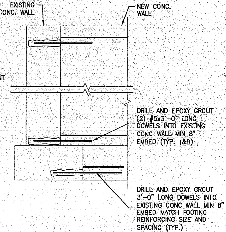
3 SECTION AT EXISTING WALL SCALE: 3/4" = 1'-0"
