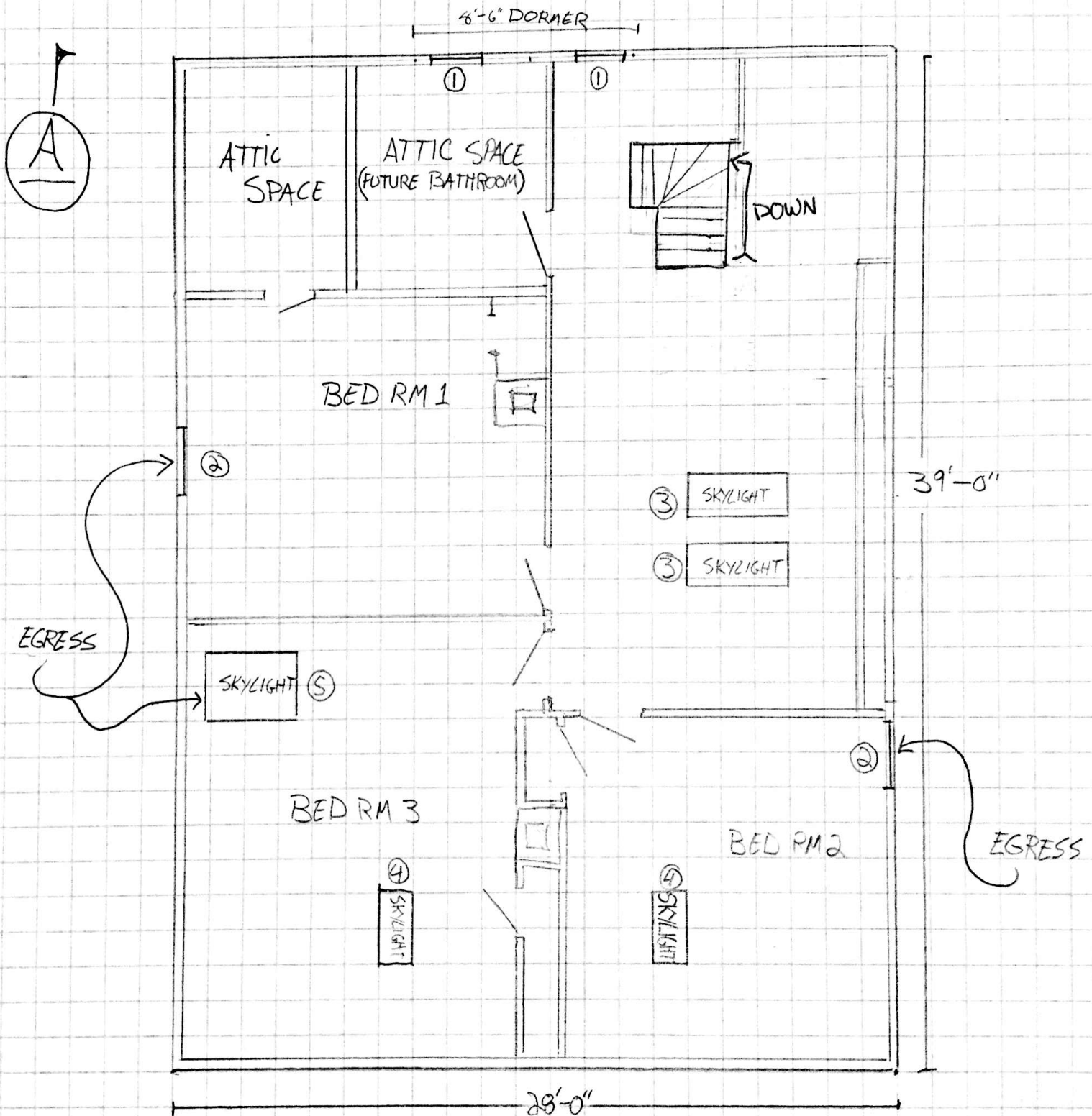
THIRD FLR PLAN SCALE 3/16" = 1'-0"
