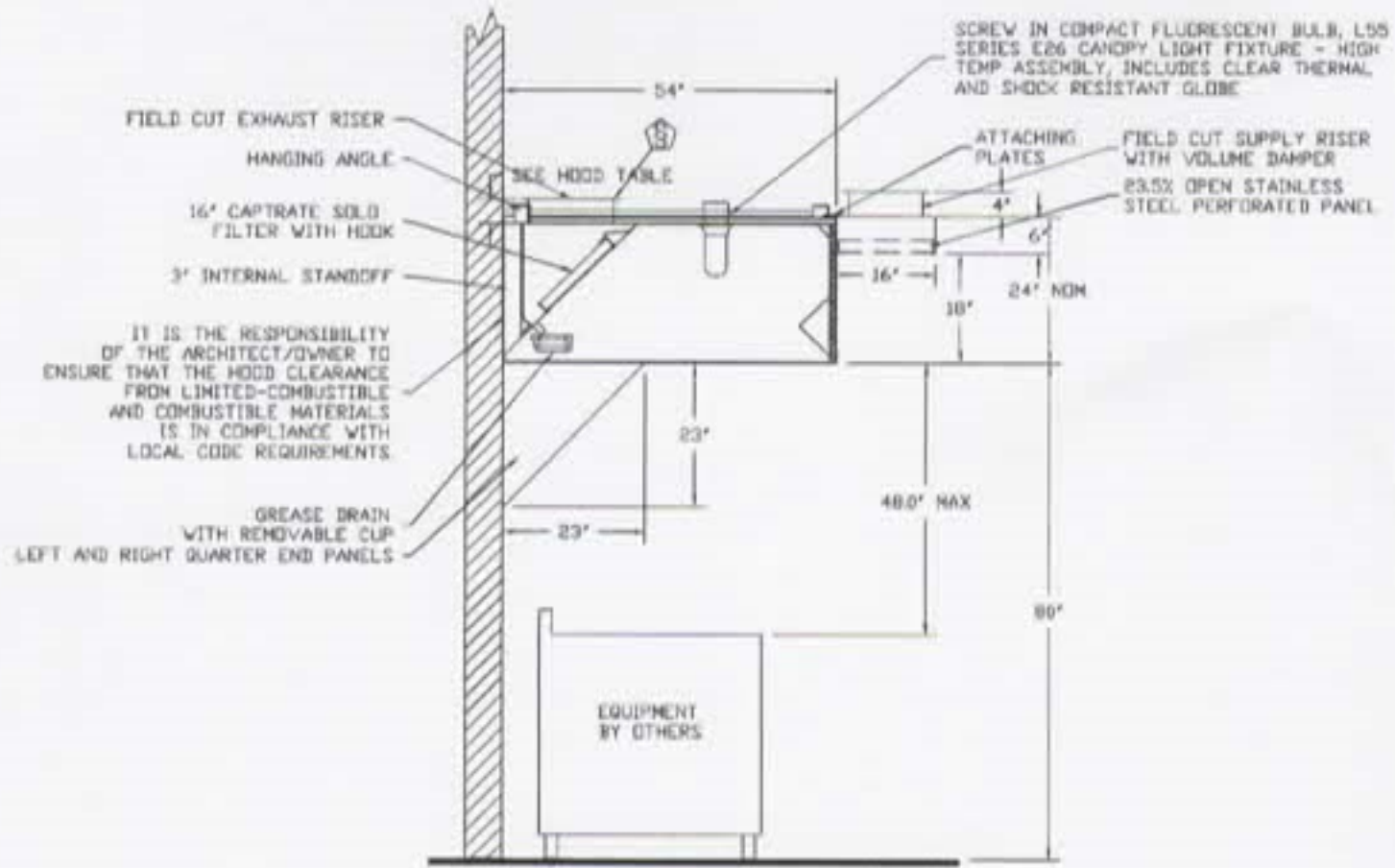
SECTION VIEW - MODEL 5424ND-2-PSP-F HOOD - #1
