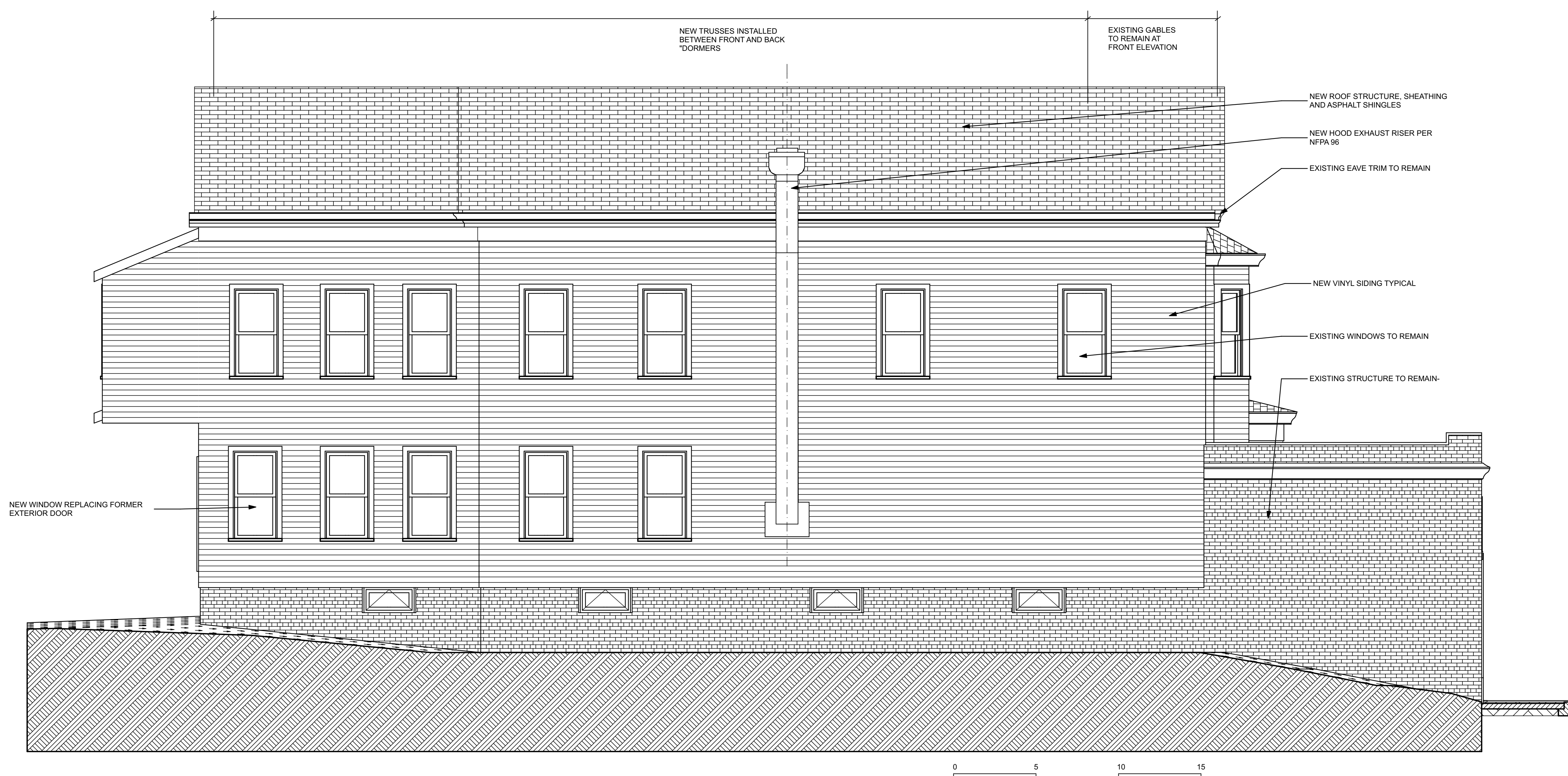
1 A2.3 SIDE ALLEY ELEVATION SCALE: 1/4" = 1'-0"
