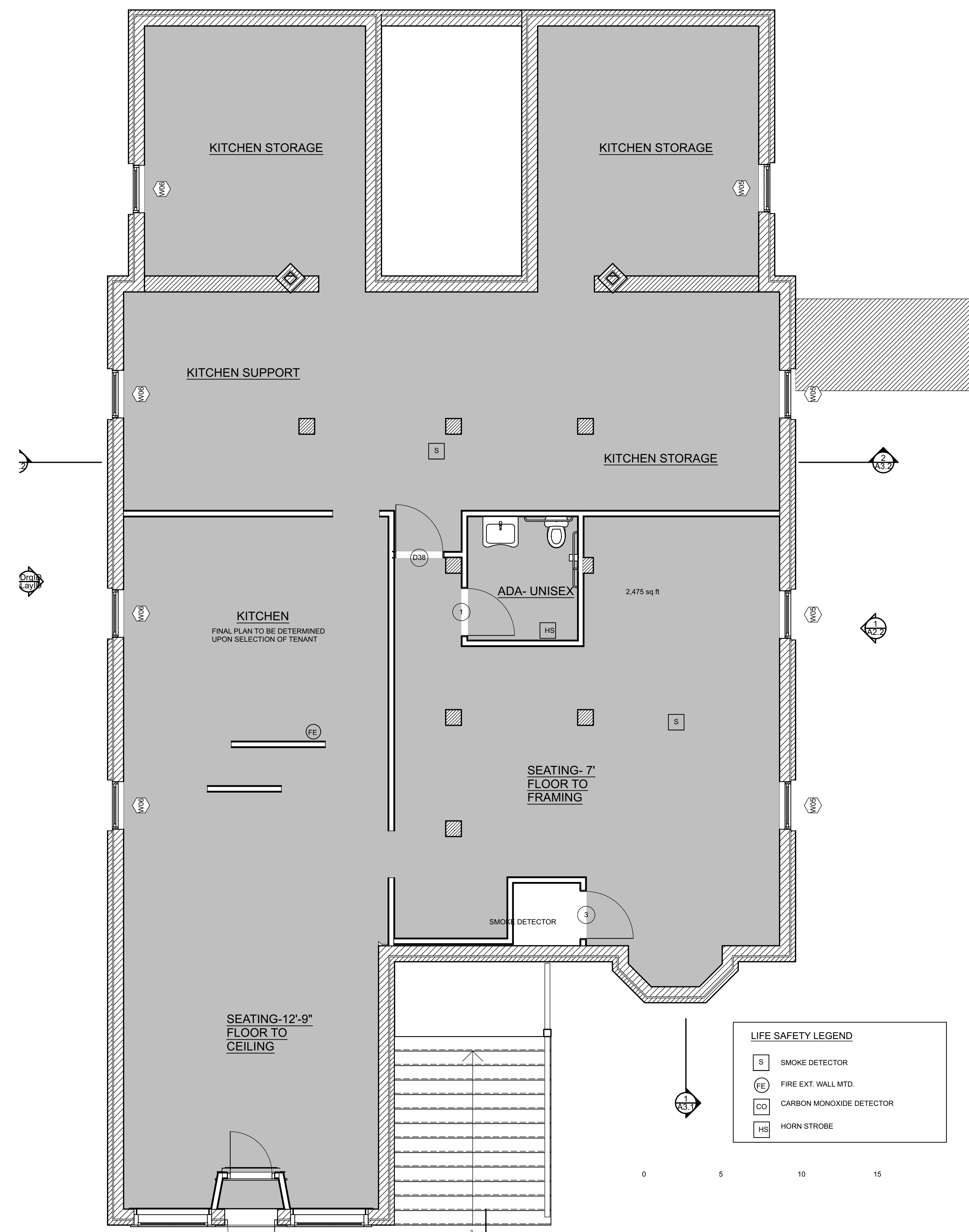
1 BASEMENT LIFE SAFETY PLAN SCALE: 1/4" = 1'-0"
