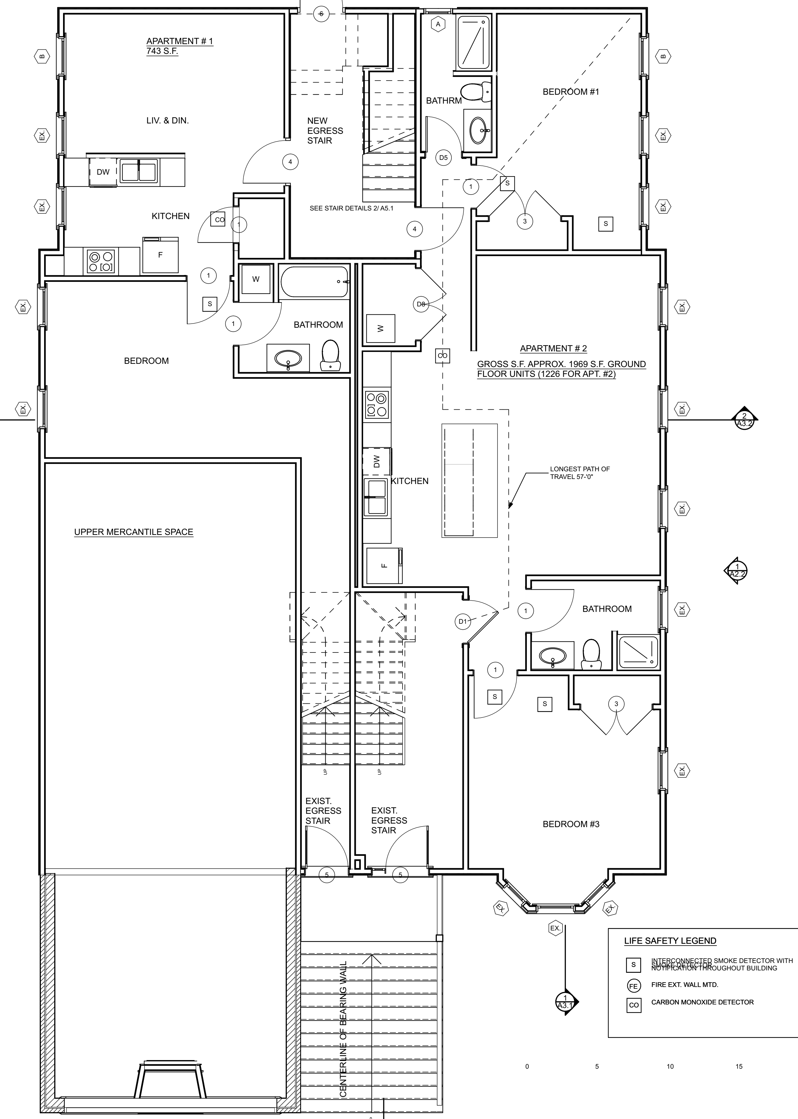
2 FIRST FLOOR LIFE SAFETY PLAN SCALE: 1/4" = 1'-0"
