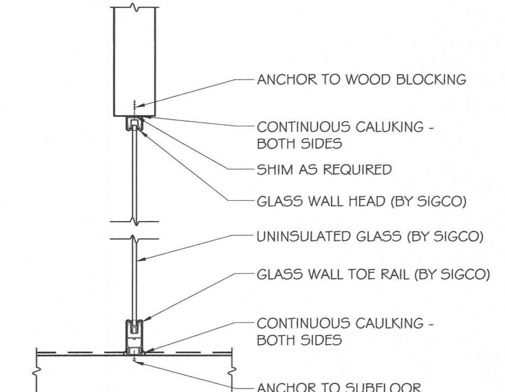
3 WALL TYPE 3
