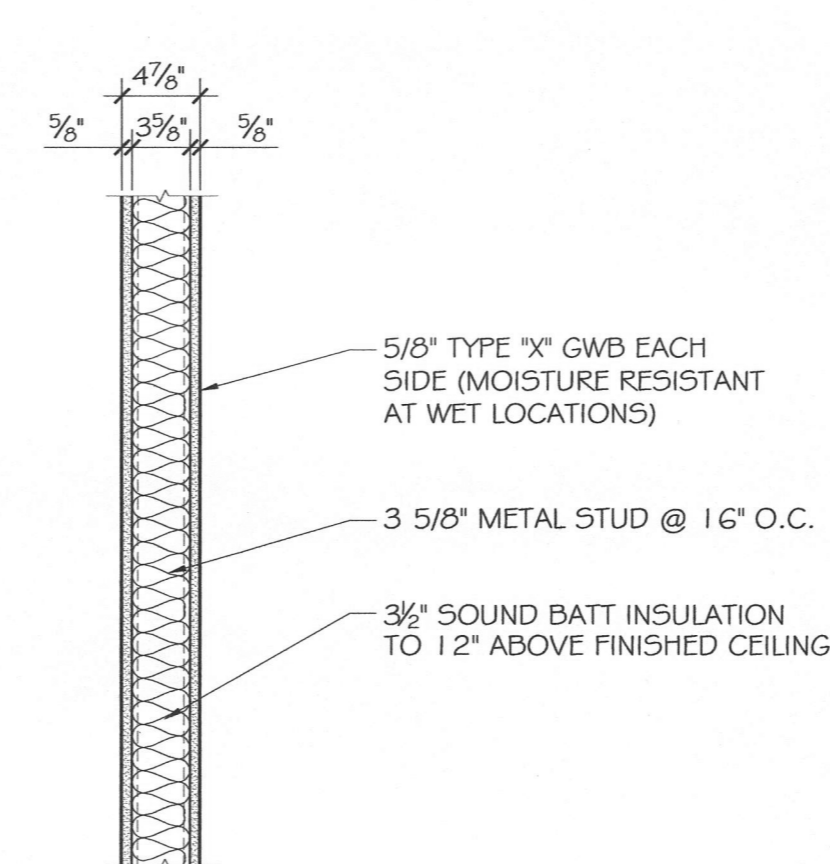
1 WALL TYPE 1
