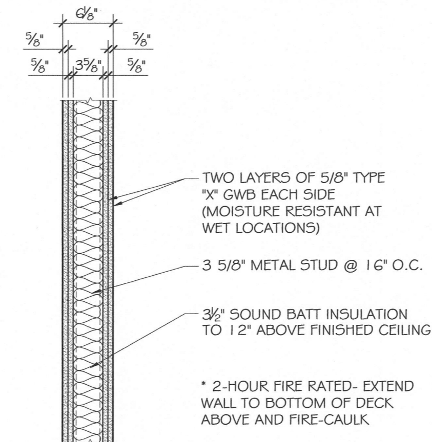
2 WALL TYPE 2
