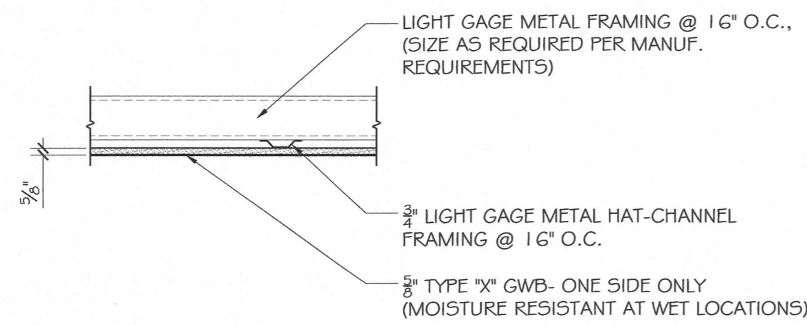
1 CEILING TYPE 1 - GWB
