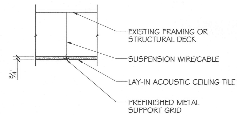
2 CEILING TYPE 2 - ACT
