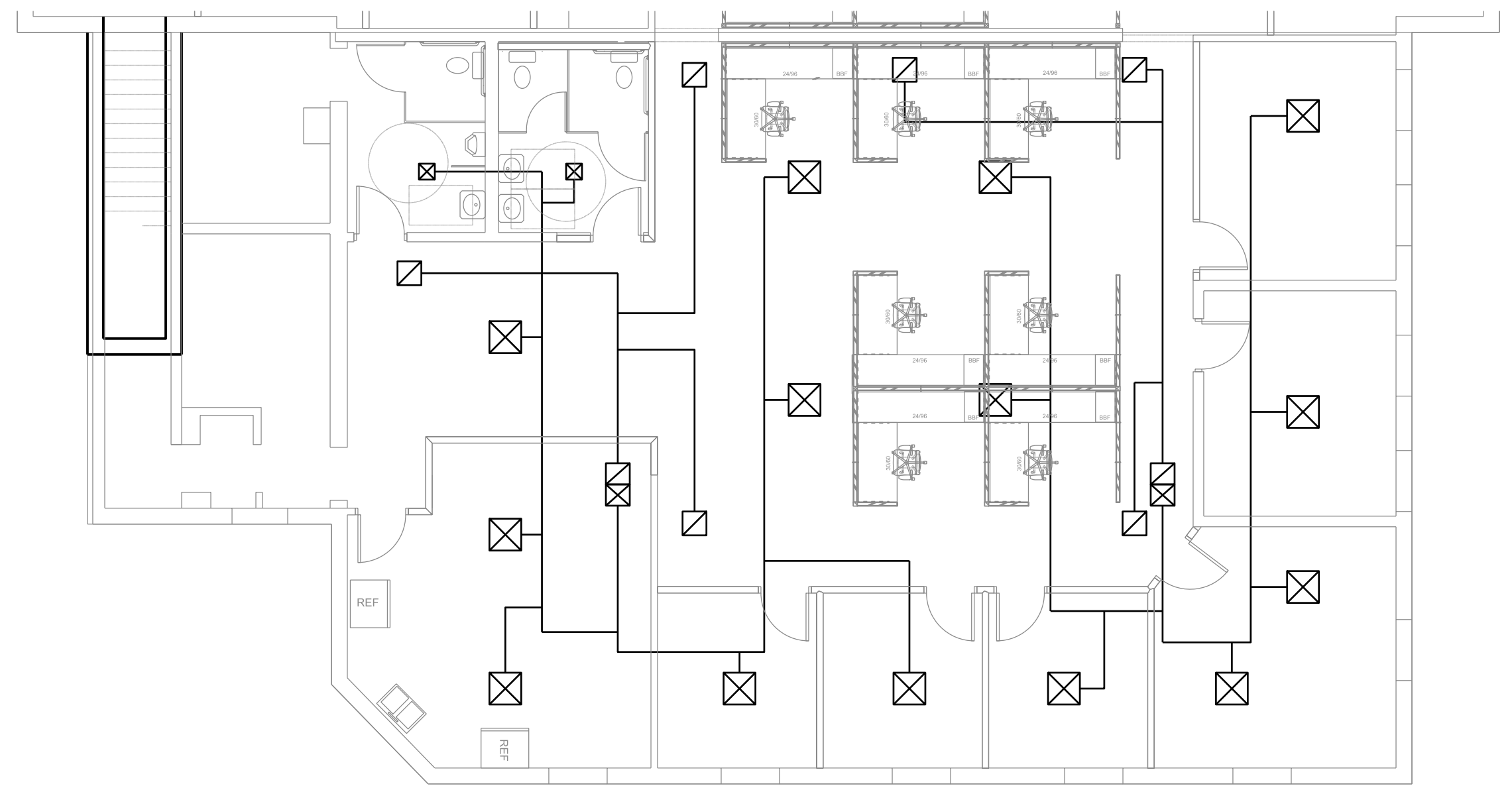
SECOND FLOOR MECHANICAL PLAN SCALE - 1/8" = 1'-0"
