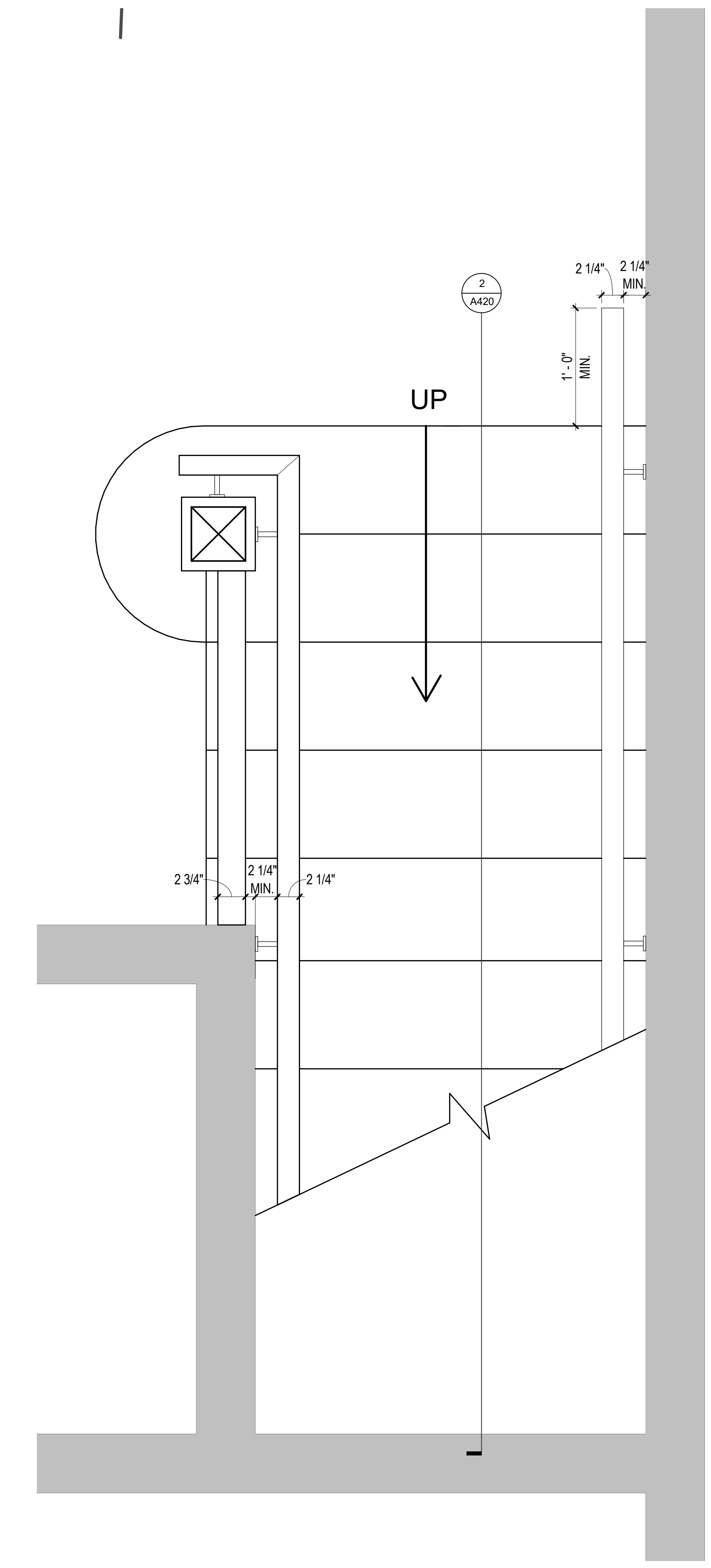
1 PLAN DETAIL @ STAIR 1 1/2" = 1'-0"
