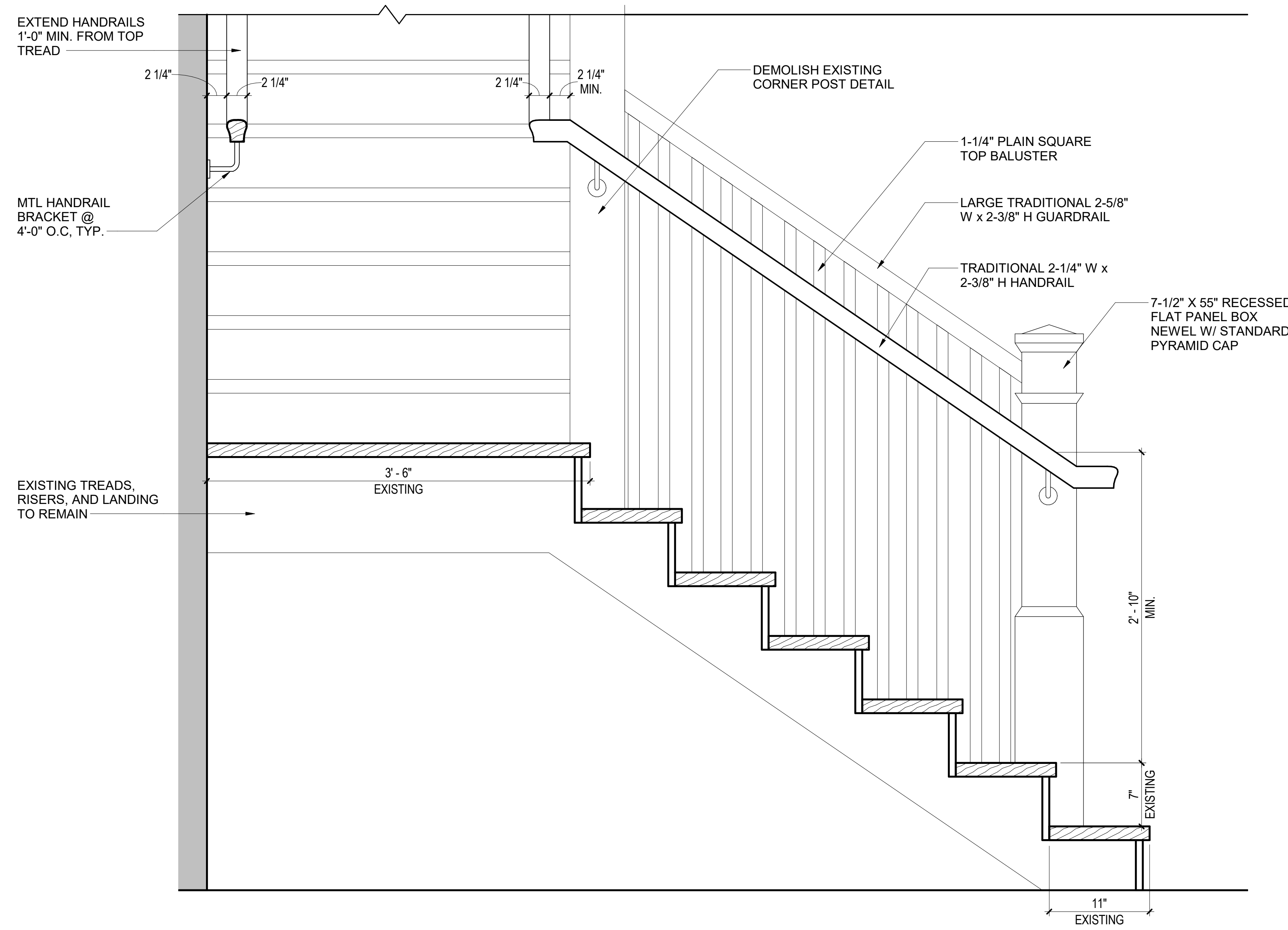
2 SECTION DETAIL @ STAIR 1 1/2" = 1'-0"
