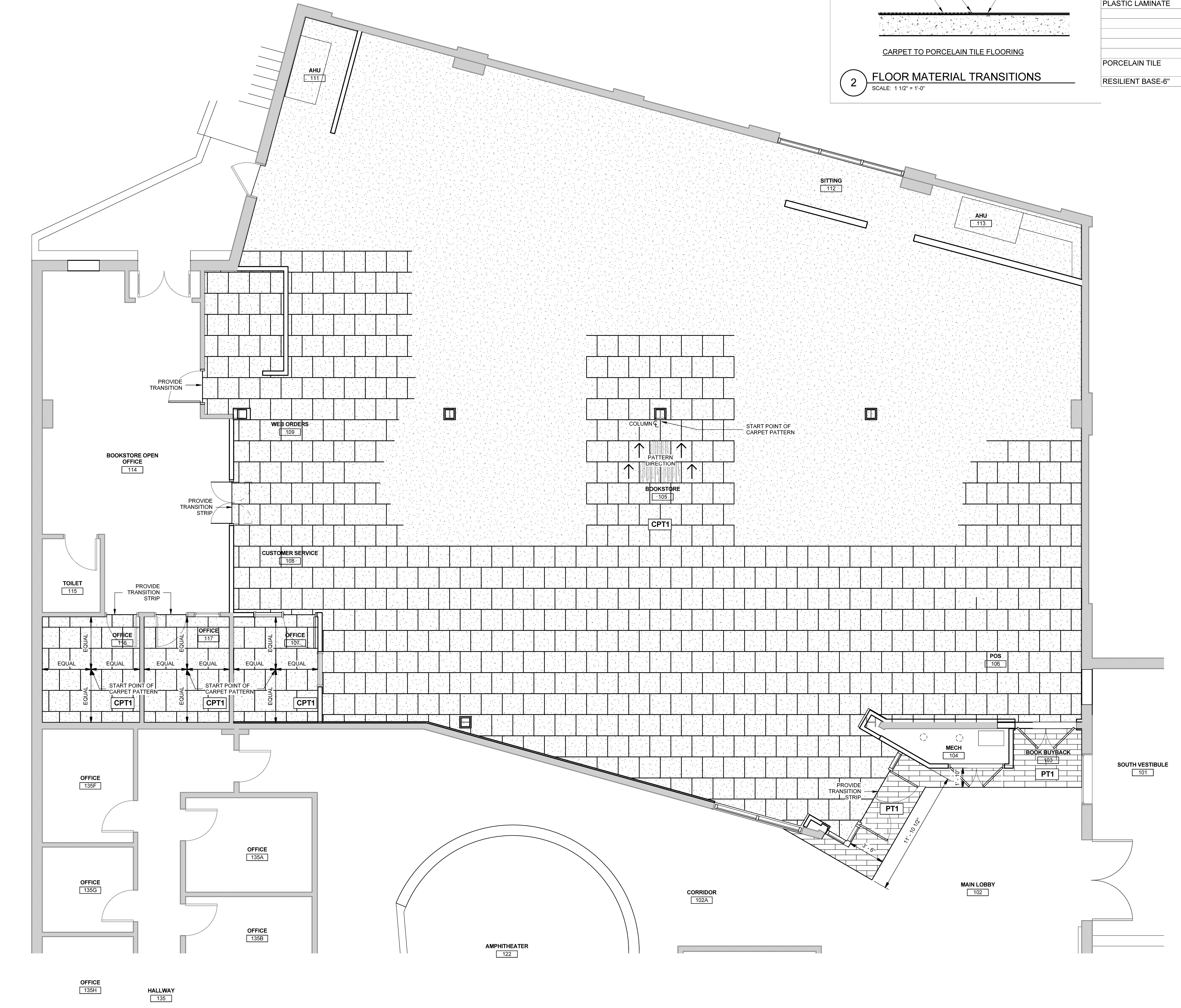
1 FIRST FLOOR MATERIALS PLAN SCALE: 1/4" = 1'-0"
