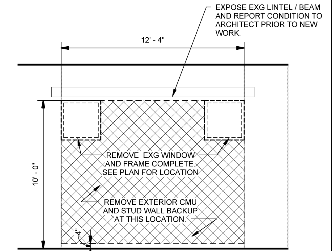
B1 ALTERNATE #2 -EXT. WALL DEMO SCALE: 1/4" = 1'-0"
