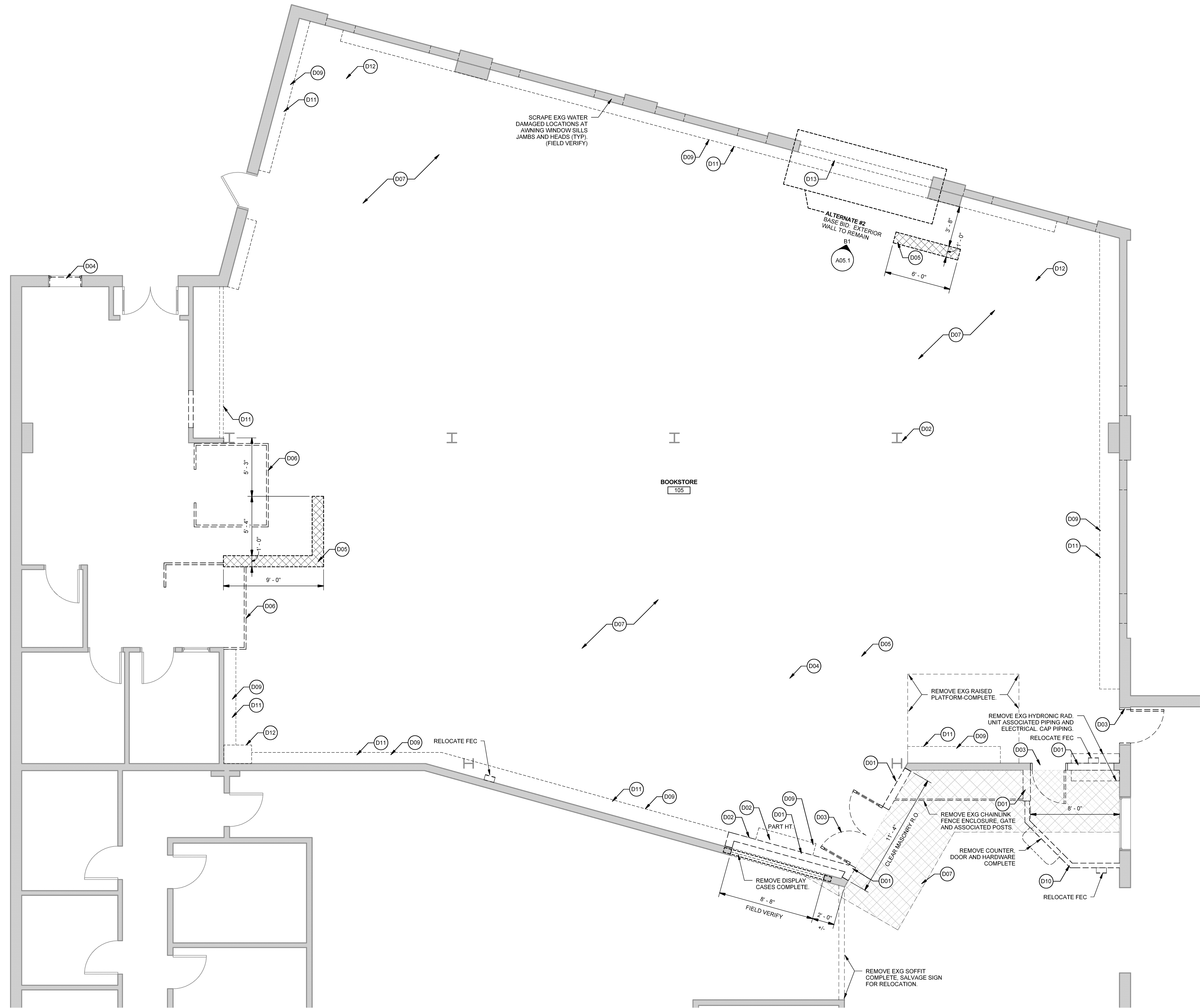
A1 FIRST FLOOR DEMOLITION PLAN SCALE: 1/4" = 1'-0"
