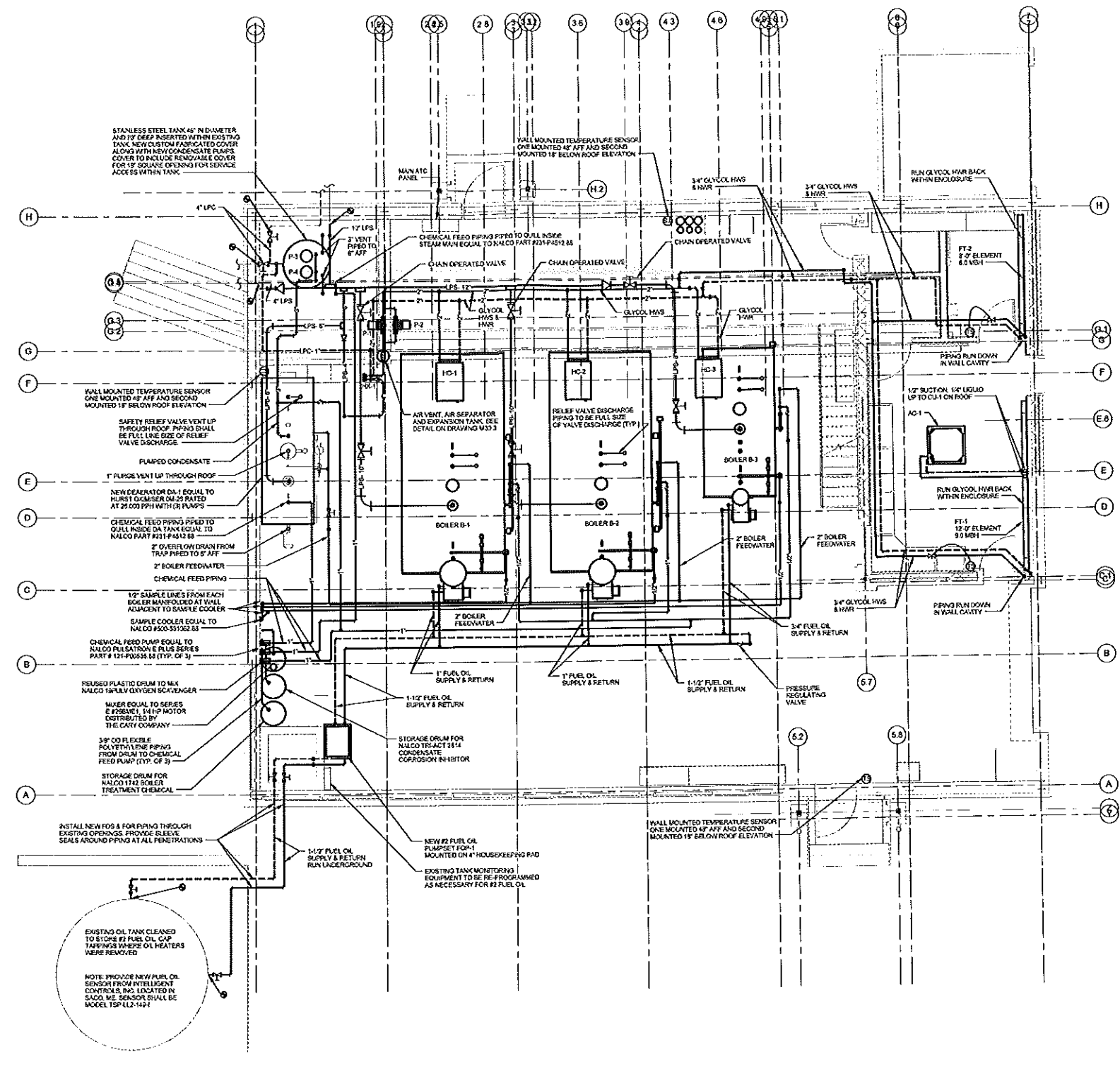
1 FIRST FLOOR PIPING SCALE 1/4" = 1'-0"
