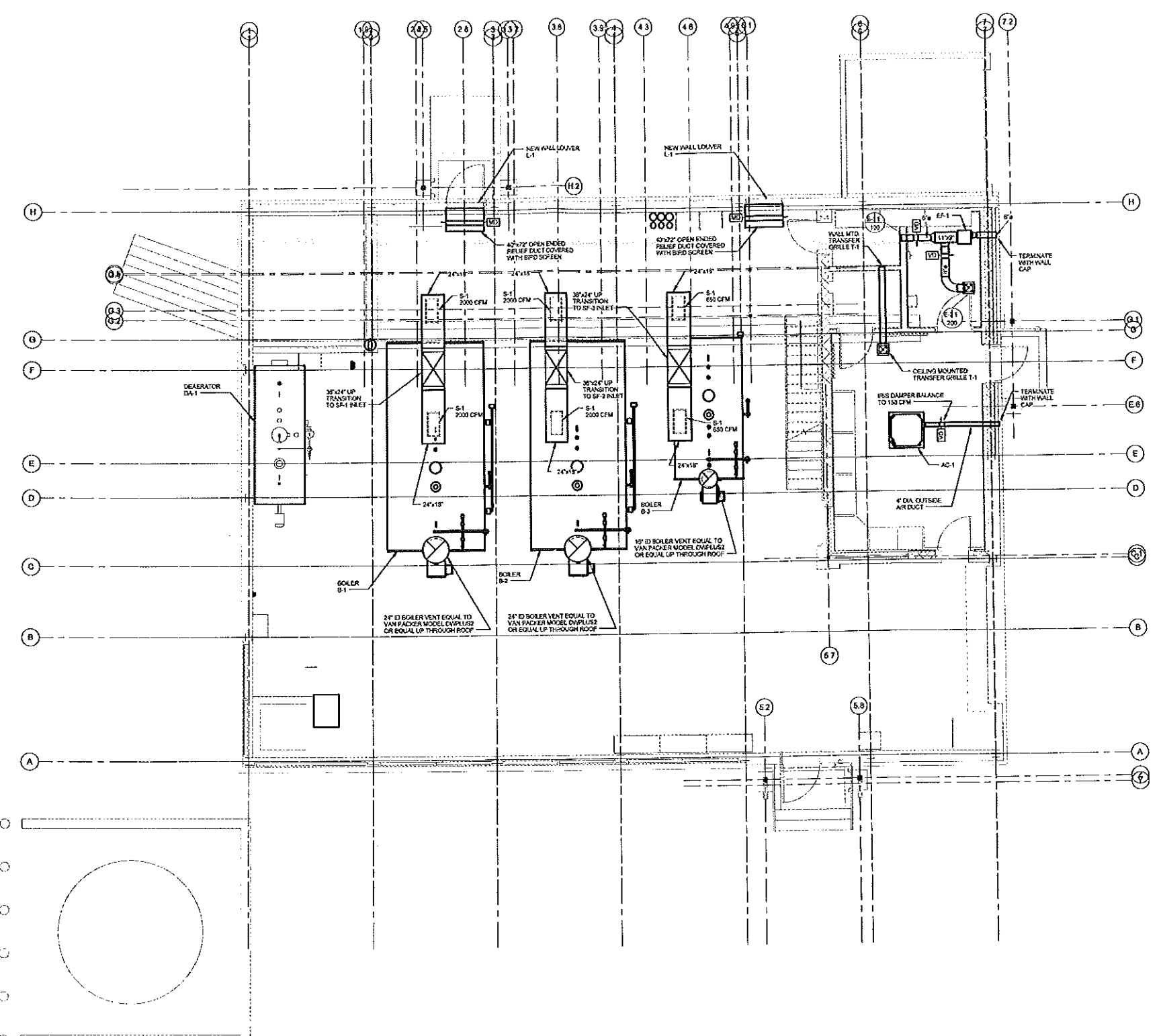
1 FIRST FLOOR DUCTWORK SCALE: 1/4" = 1'-0"
