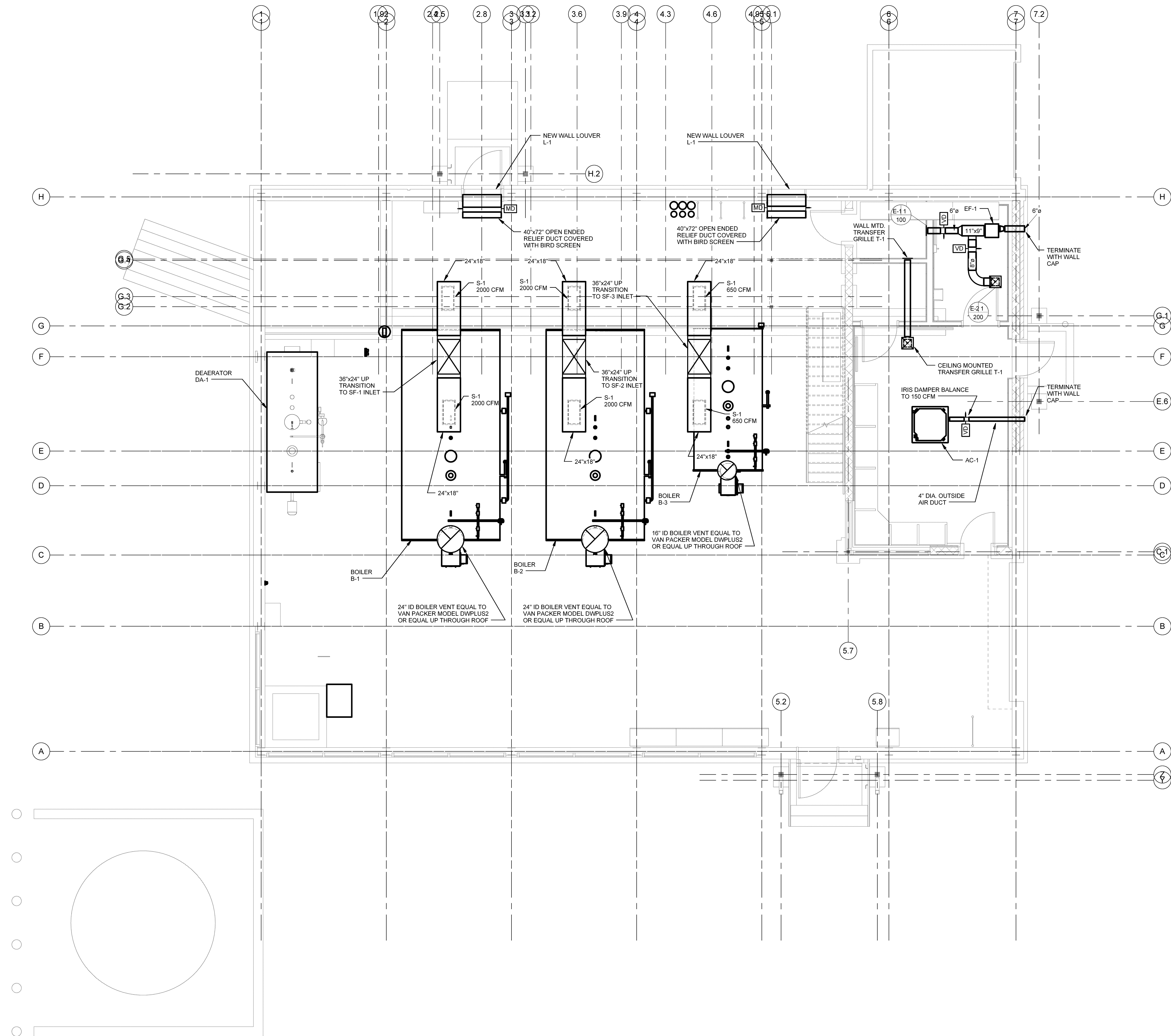
1 FIRST FLOOR DUCTWORK SCALE: 1/4" = 1'-0"
