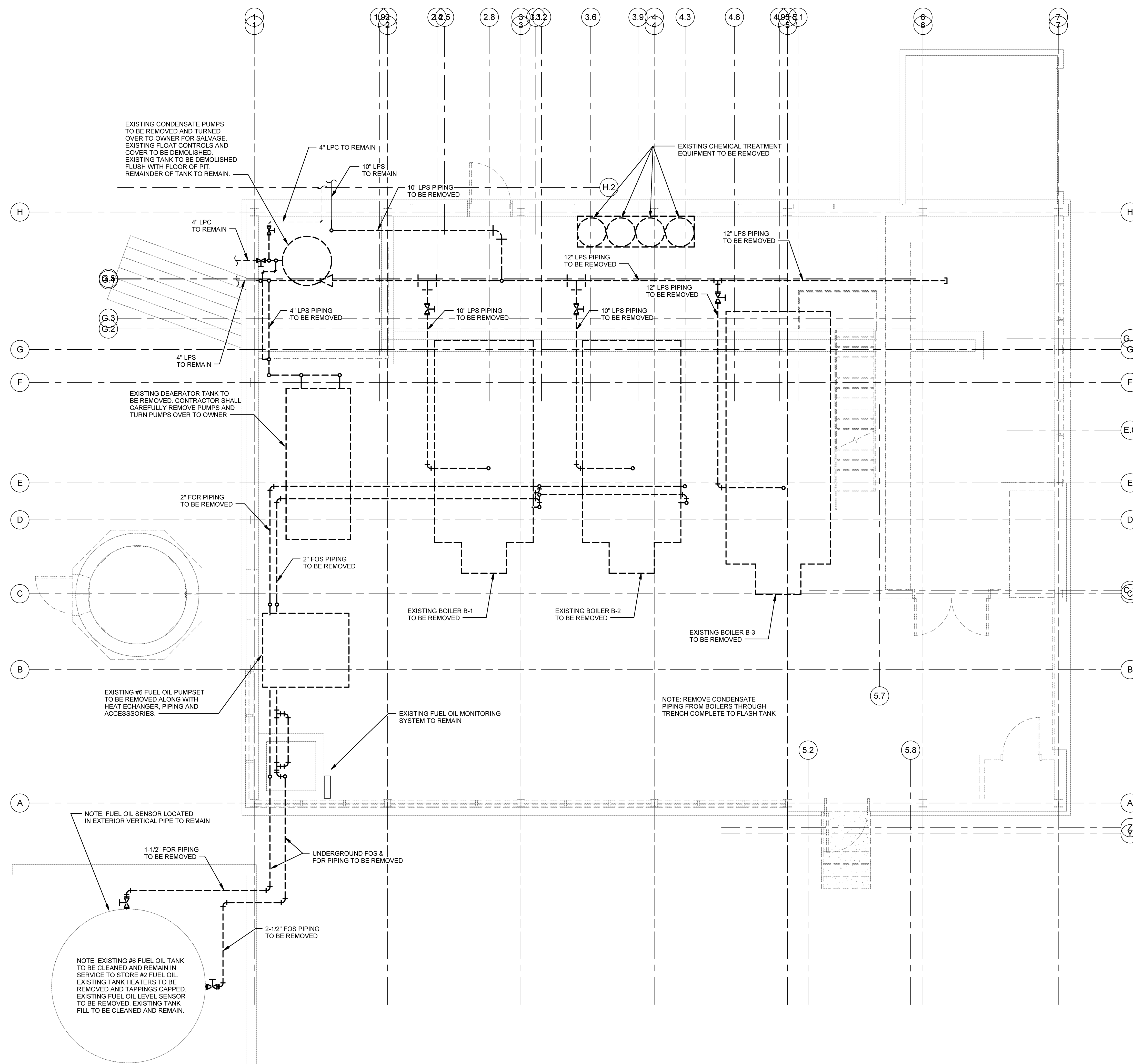
1 FIRST FLOOR PIPING DEMOLITION SCALE: 1/4" = 1'-0"
