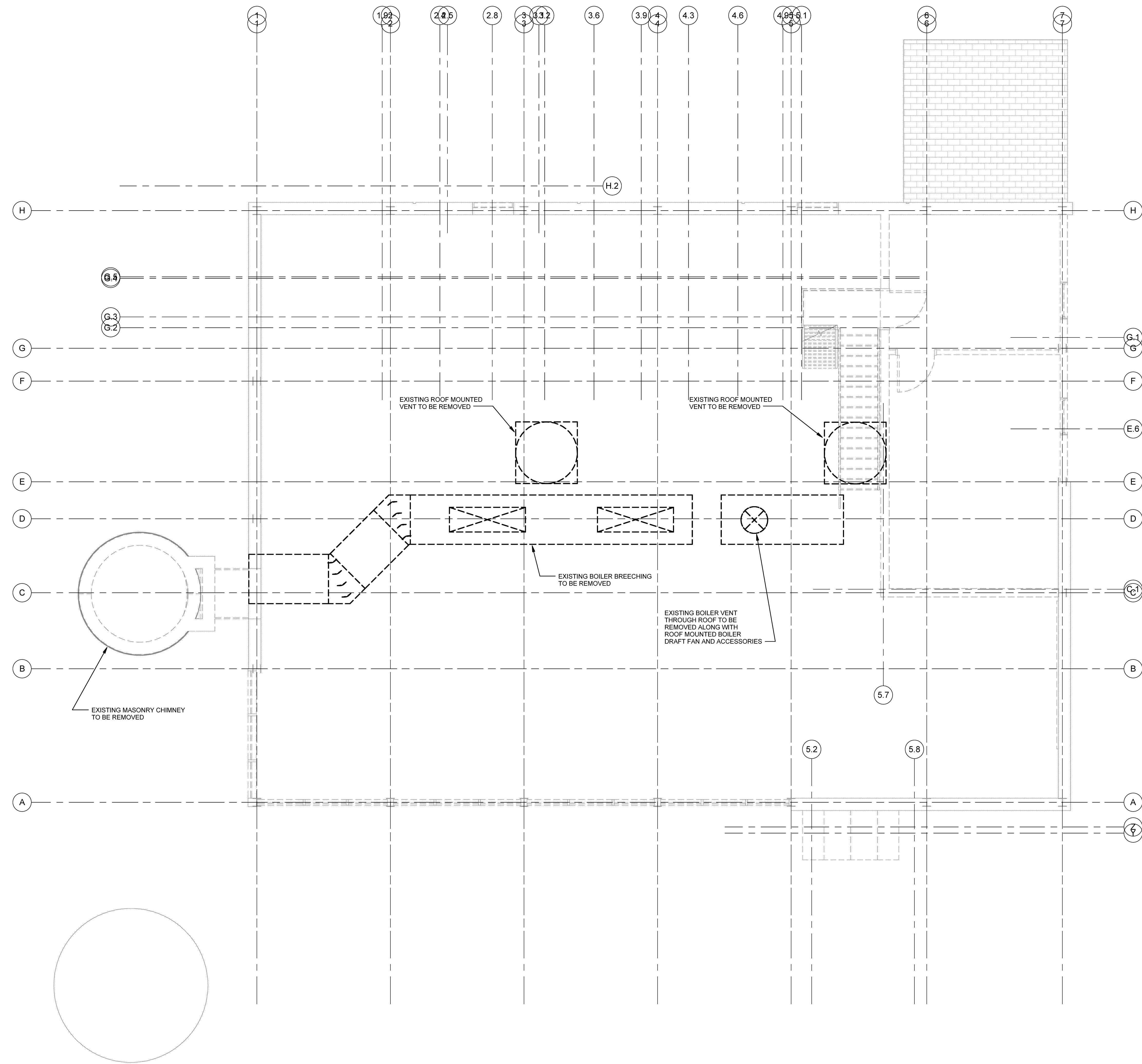
1 SECOND FLOOR DUCT DEMOLITION SCALE: 1/4" = 1'-0"
