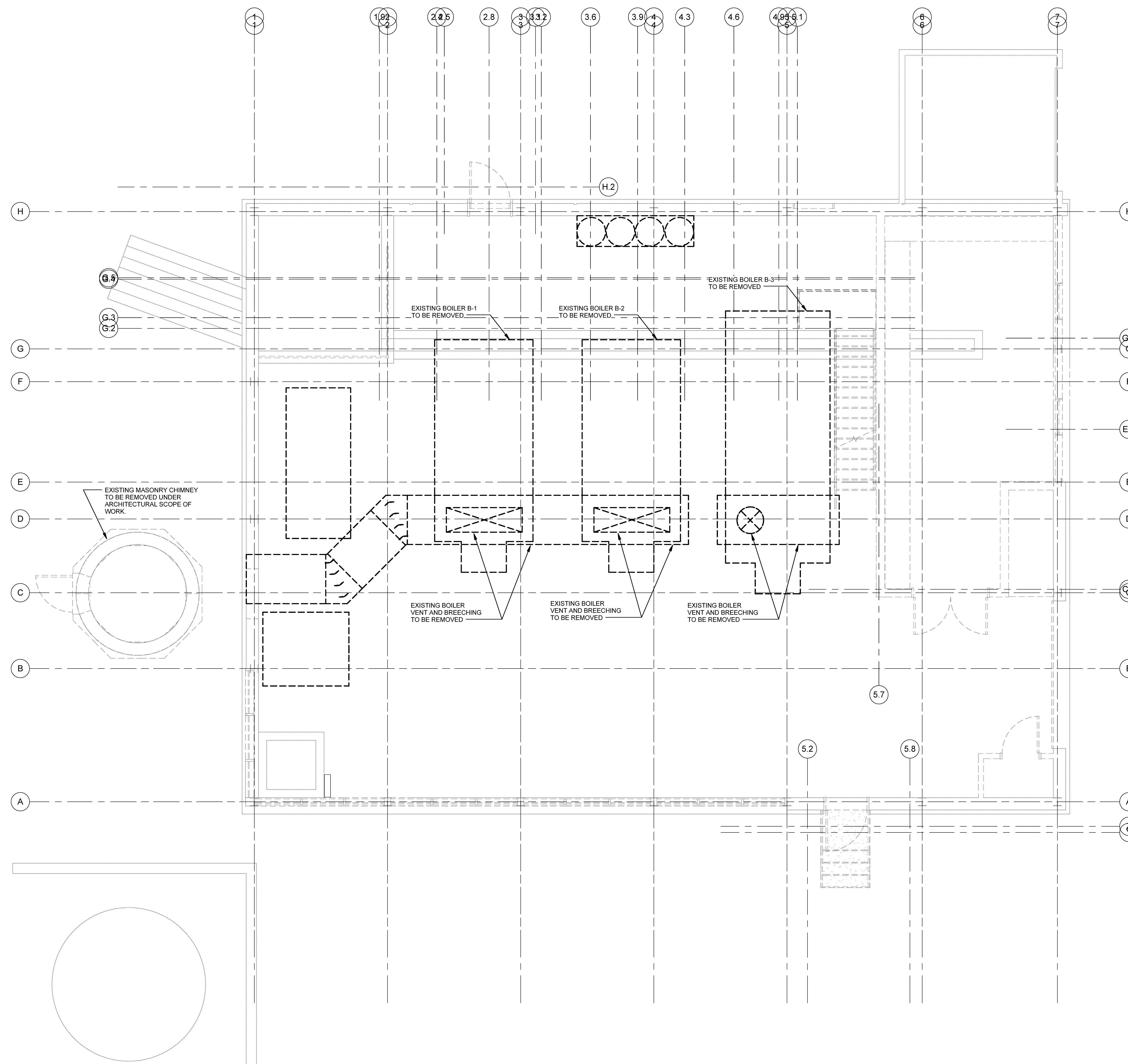
1 FIRST FLOOR DUCT DEMOLITION SCALE: 1/4" = 1'-0"
