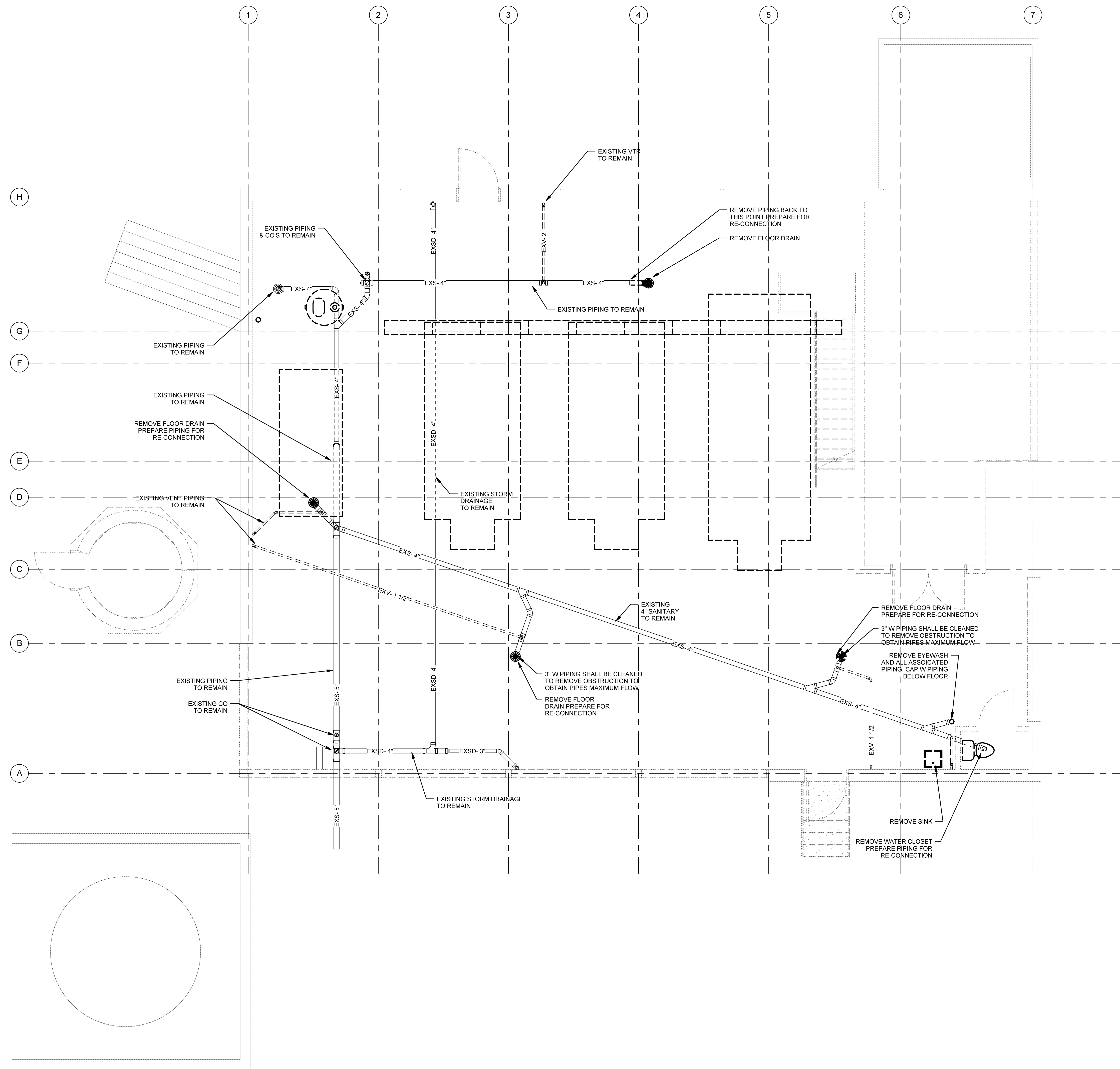
1 FIRST FLOOR DEMOLITION UNDERSLAB DRAINAGE SCALE: 1/4" = 1'-0"
