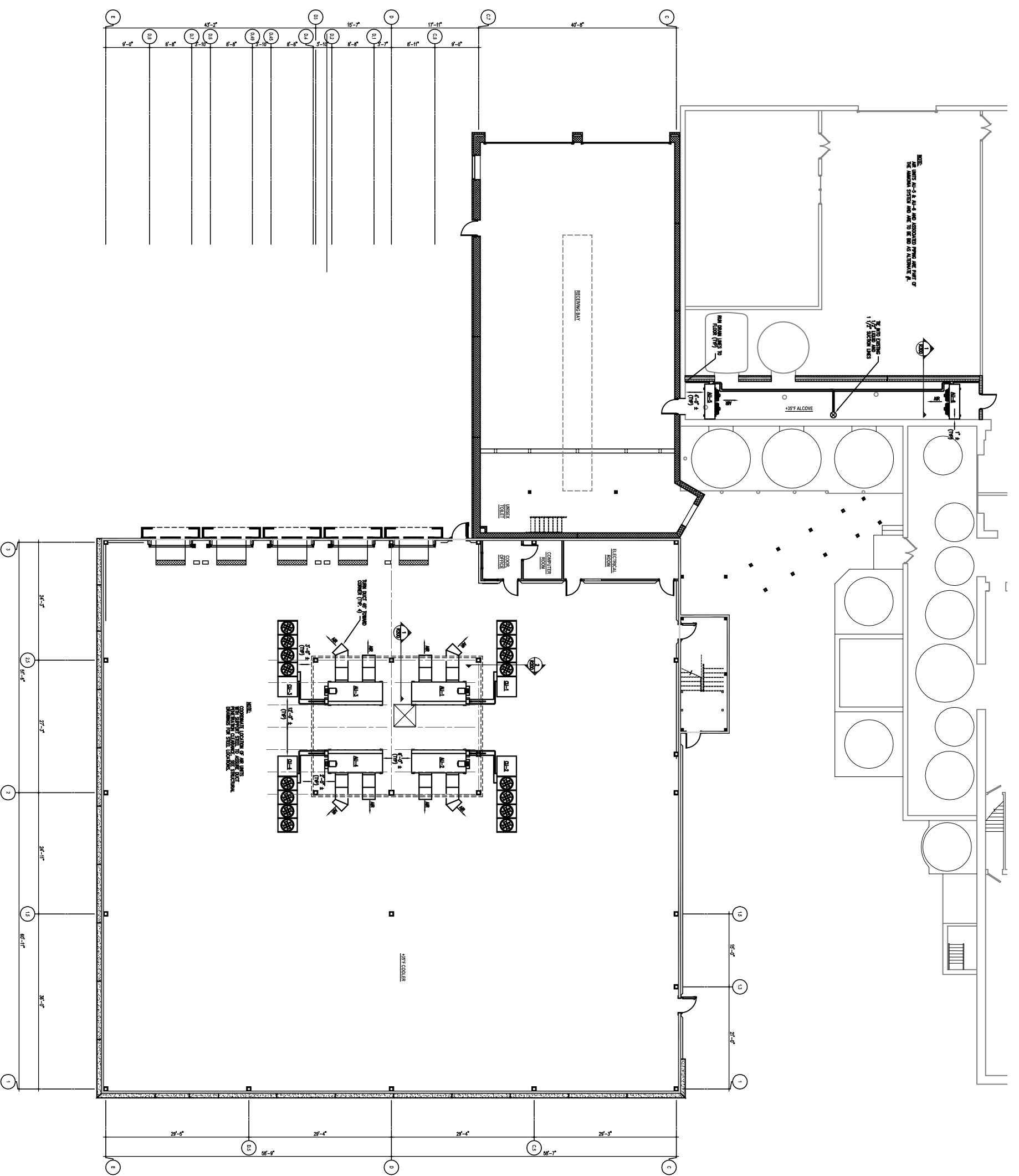
OVERALL REFRIGERATION PLAN SCALE 1/8" = 1'-0"
