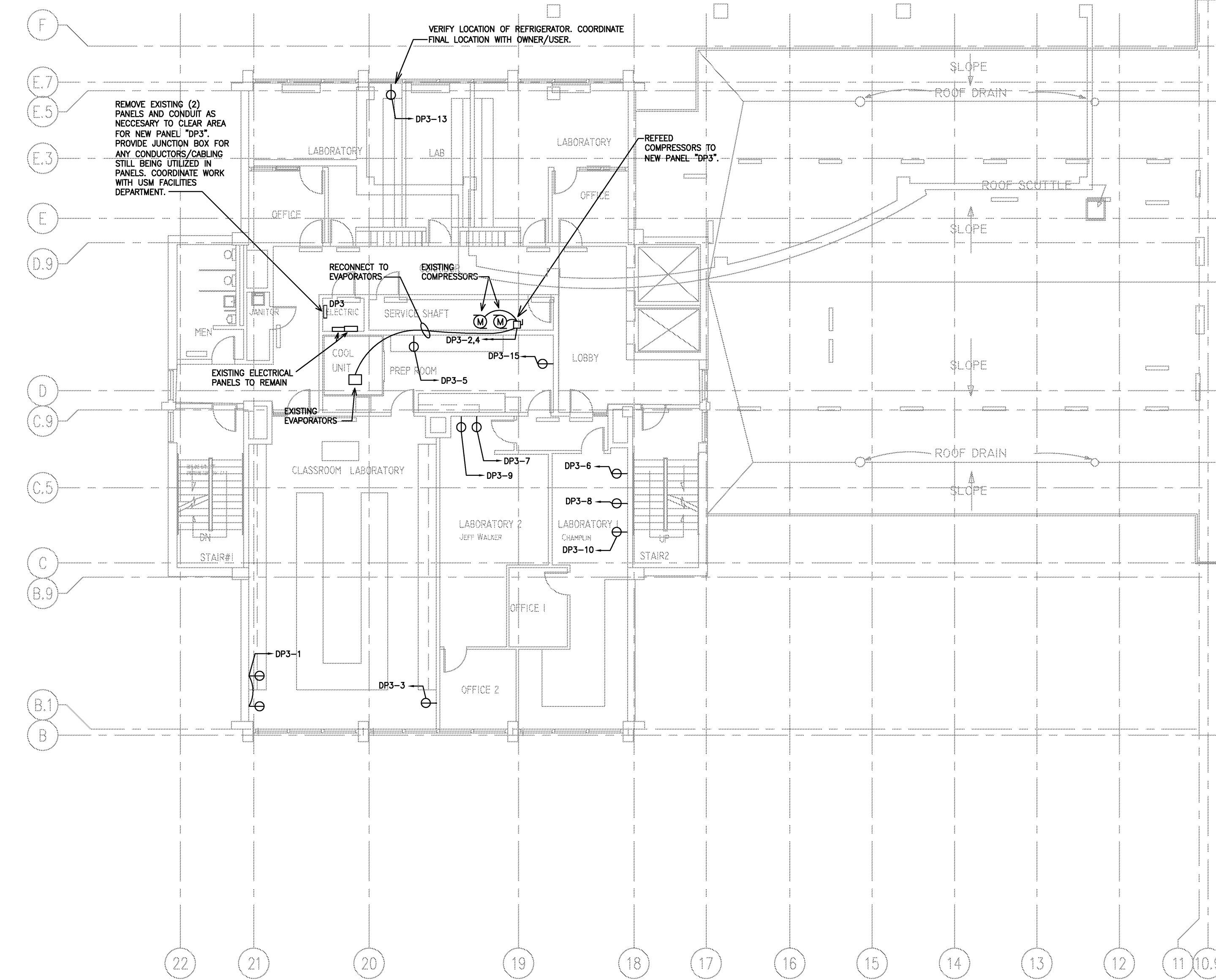
THIRD FLOOR PARTIAL PLAN — NEW WORK 3/32" = 1'-0" REF: NA A2
