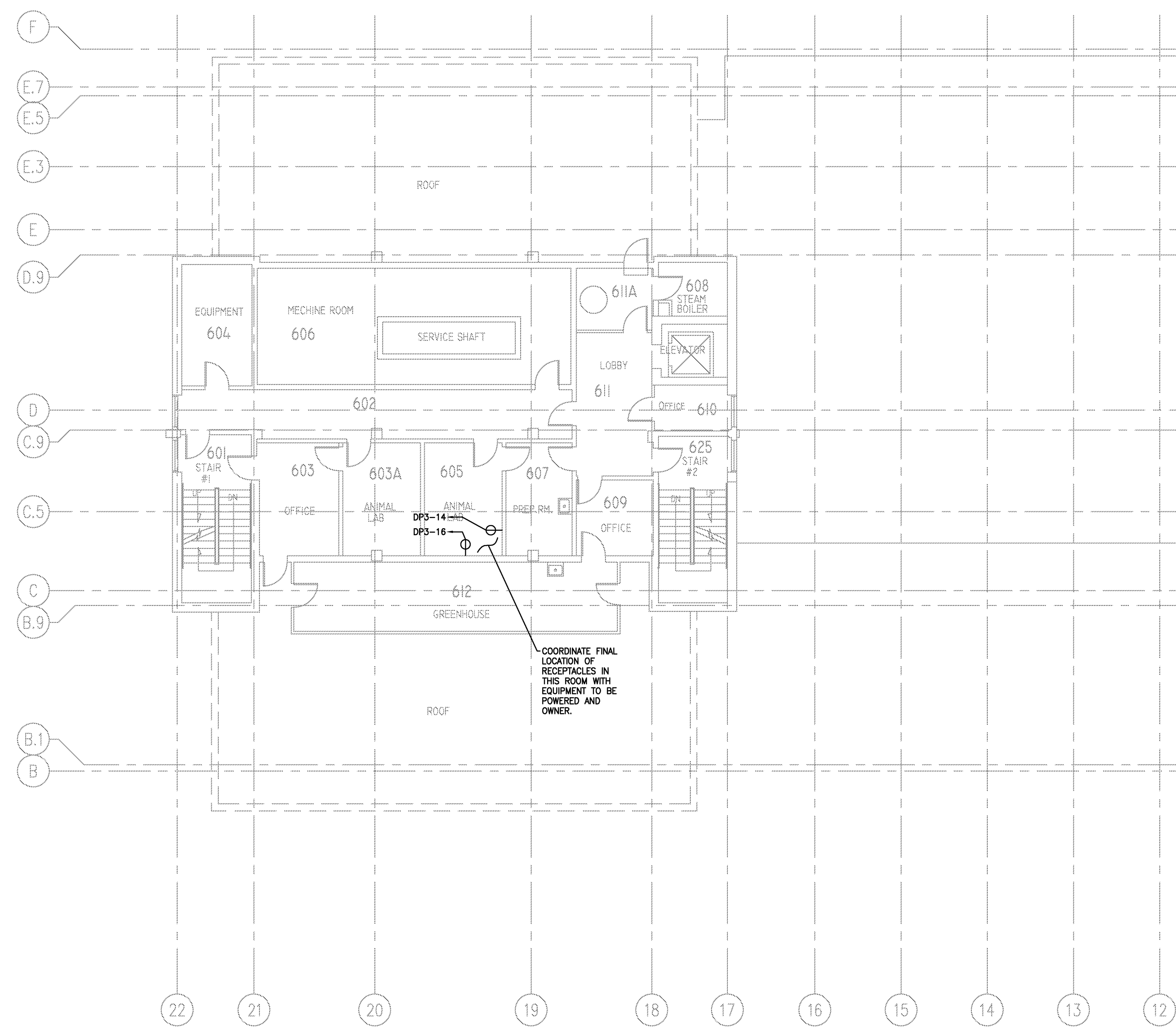
SIXTH FLOOR PARTIAL PLAN — NEW WORK 3/32" = 1'-0" REF: NA A4
