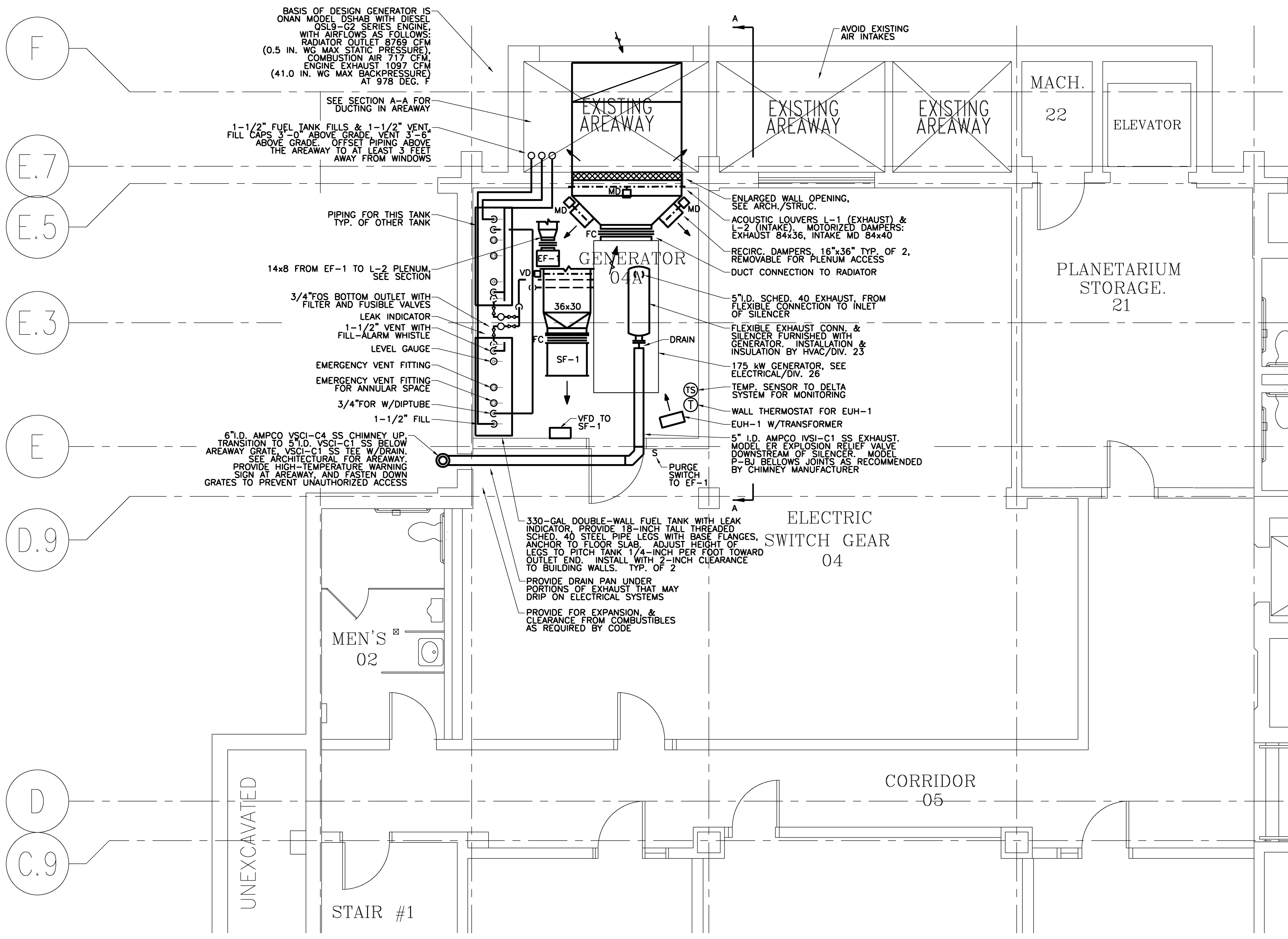
BASEMENT FLOOR PLAN 1/4" = 1'-0" REF: NA A1
