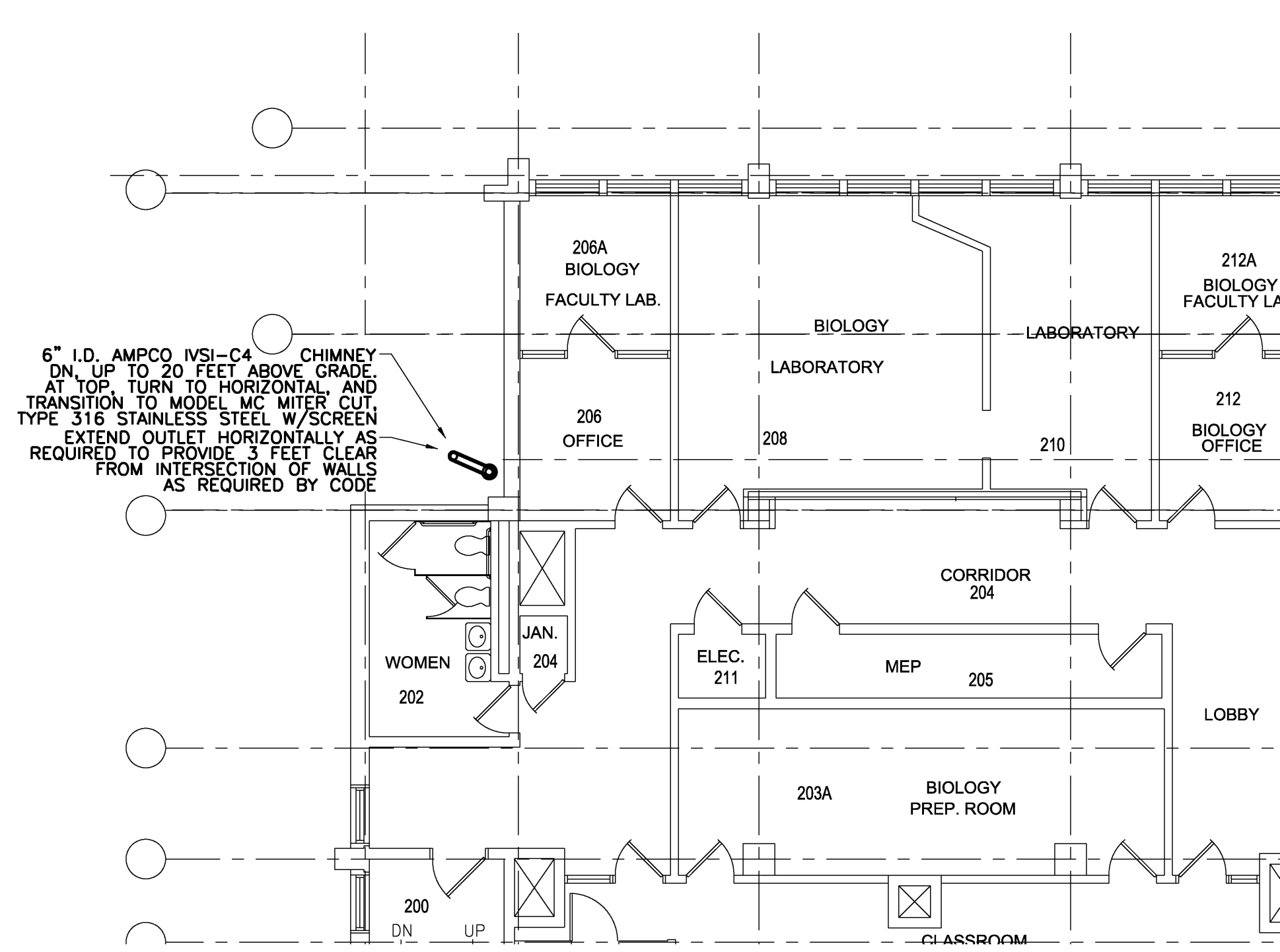
SECOND FLOOR PLAN 1/8" = 1'-0" REF: NA B2
