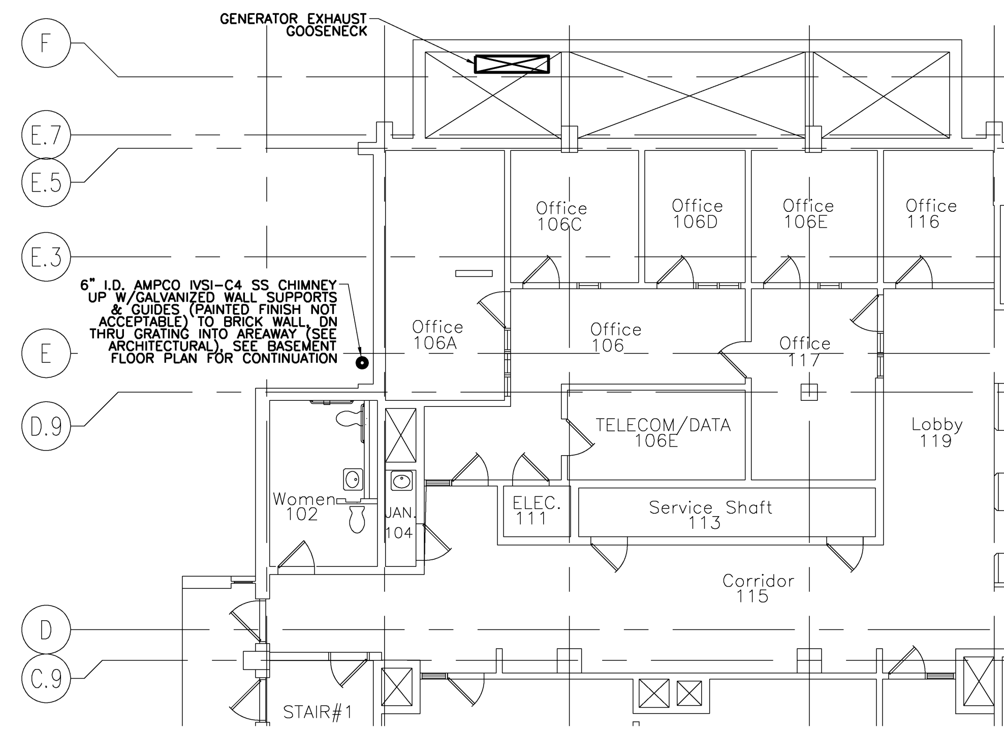
FIRST FLOOR PLAN 1/8" = 1'-0" REF: NA B1
