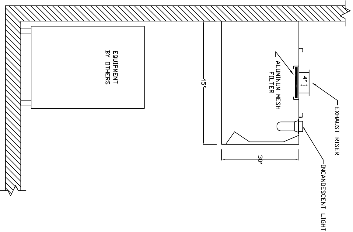
SECTION VIEW - MODEL 4530 VH1-ND
