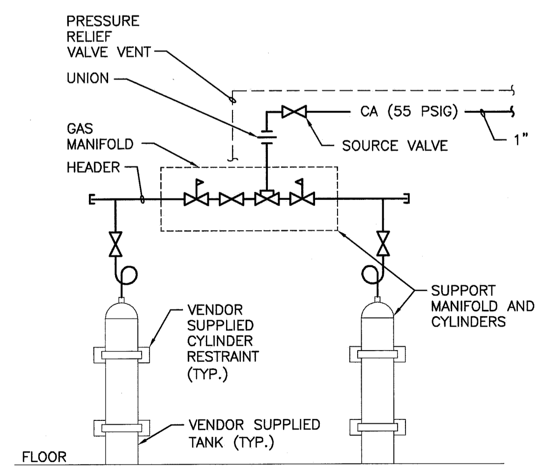
A1 CA CYLINDER DETAIL NOT TO SCALE
