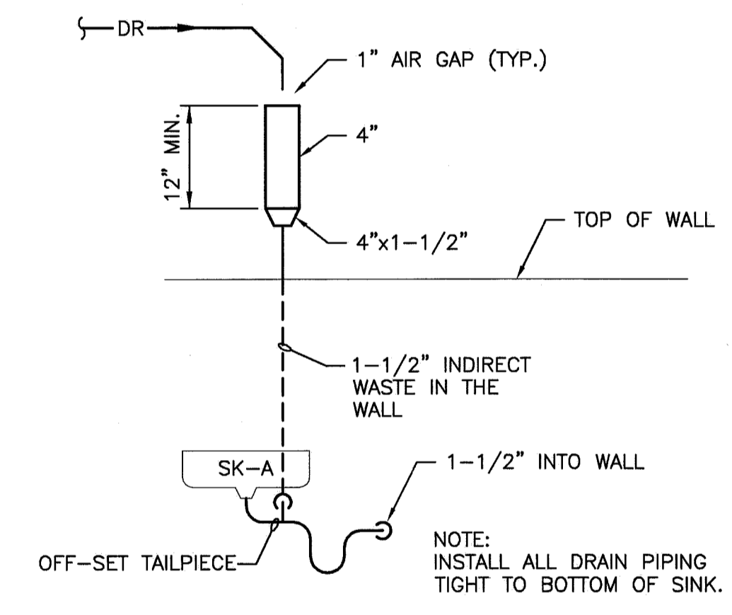
D1 INDIRECT WASTE CONNECTION NOT TO SCALE
