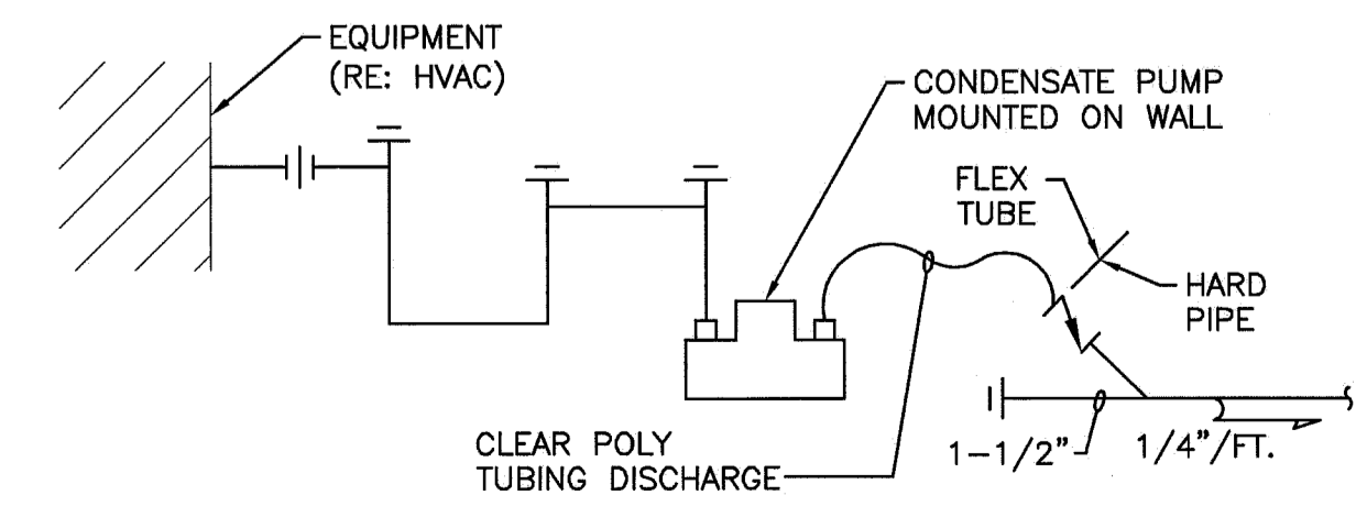
A4 CONDENSATE PUMP DETAIL NOT TO SCALE
