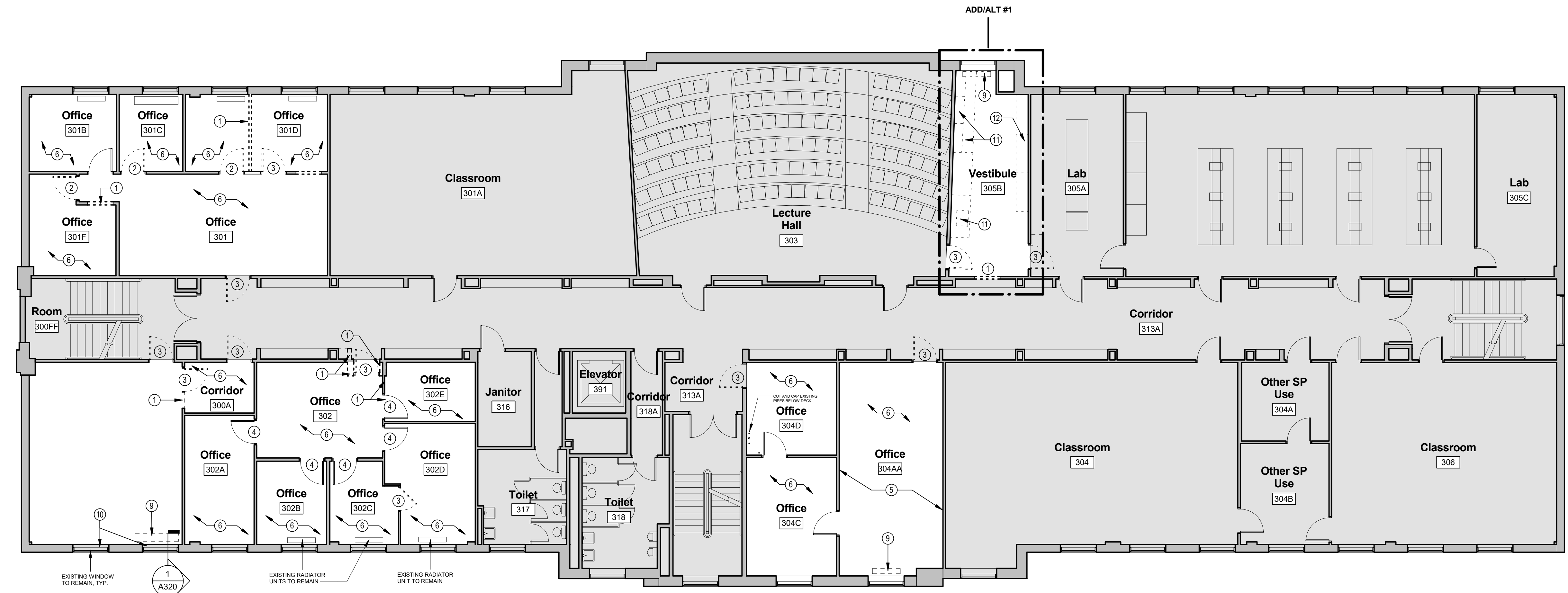
2 LEVEL 3 - Demo Ceiling Plan 1/8" = 1'-0"
