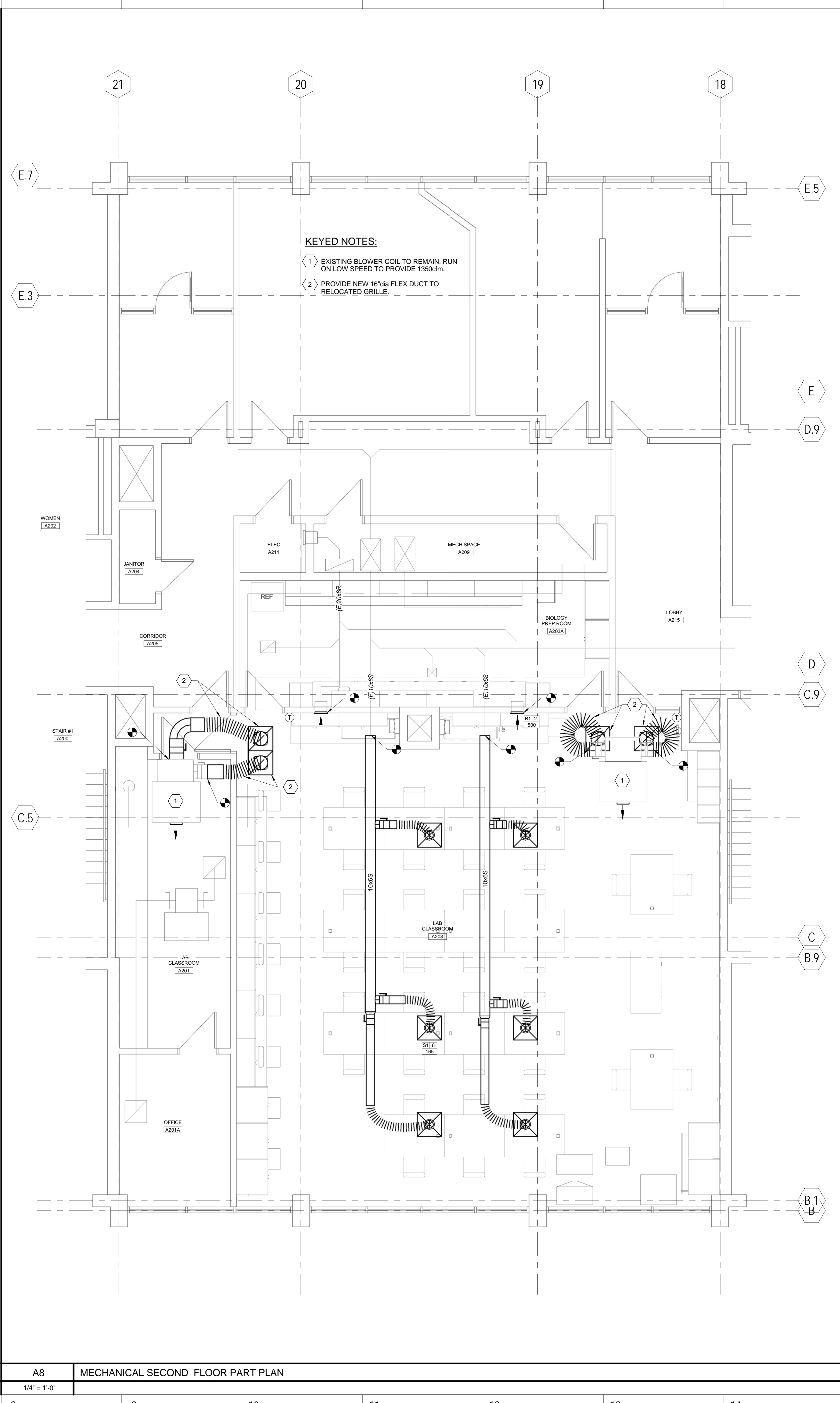
A1 MECHANICAL DEMOLITION SECOND FLOOR PART PLAN 1/4" = 1'-0"
