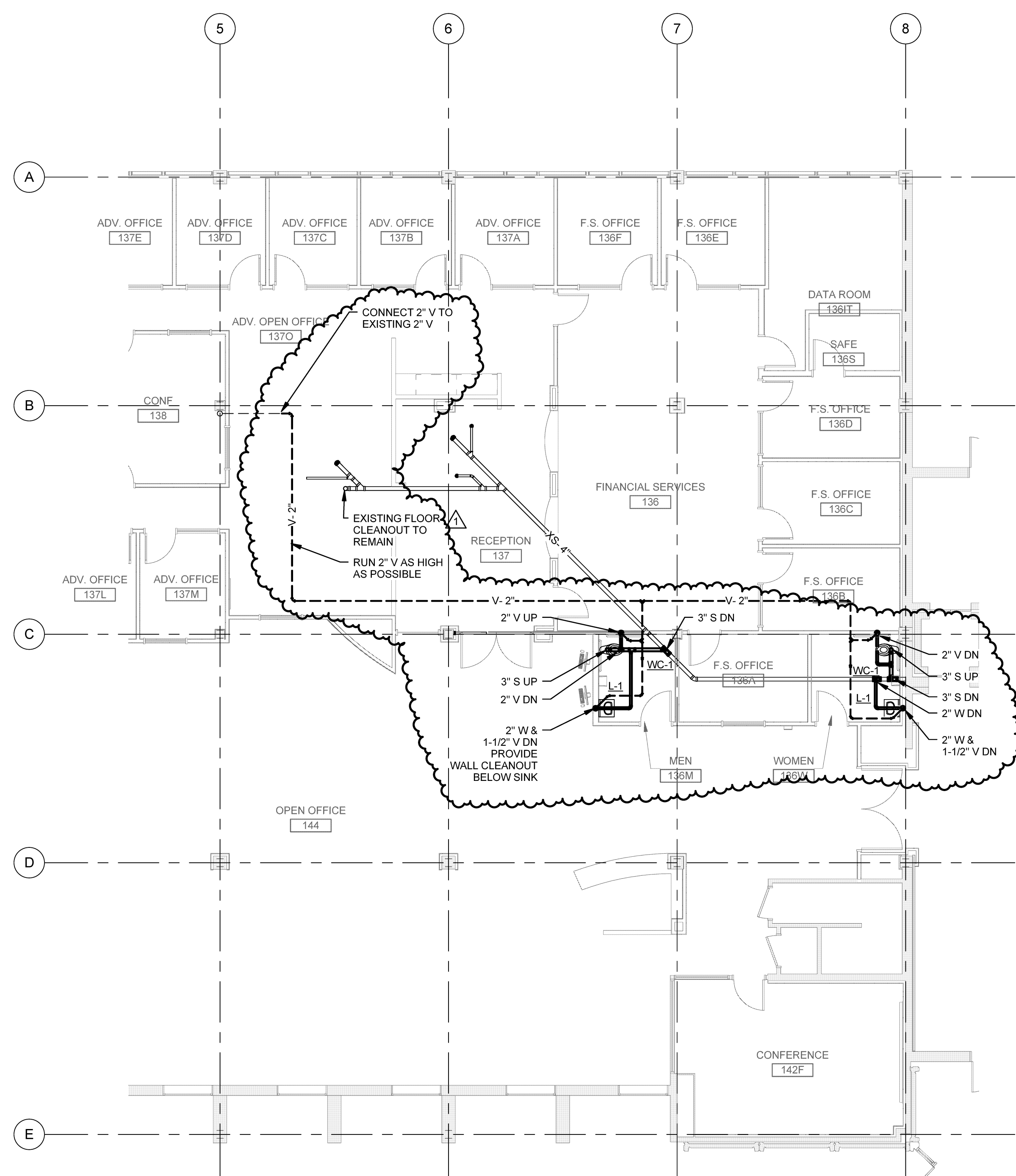
1 DRAINAGE PLAN
