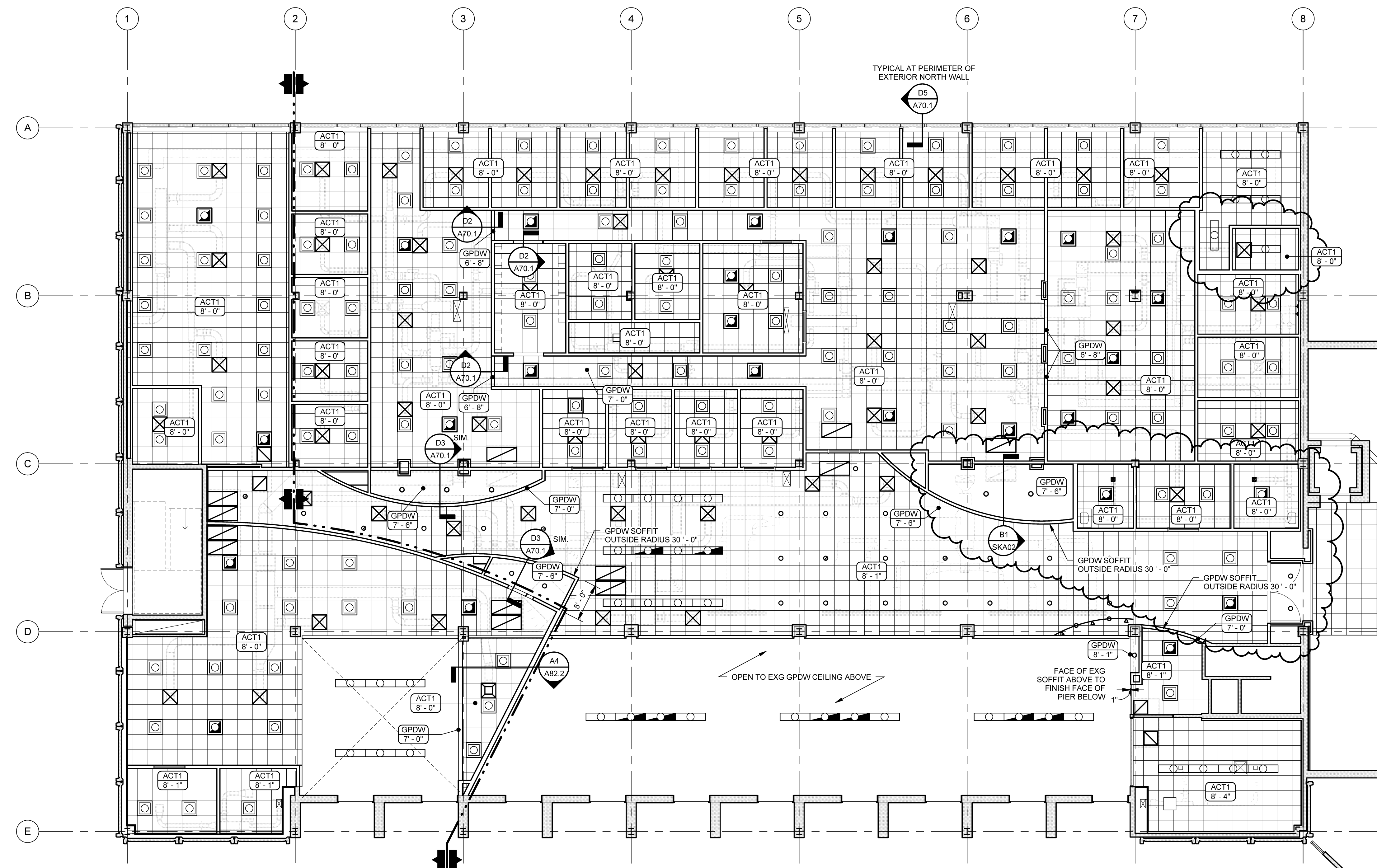
A1 FIRST FLOOR CEILING PLAN SCALE: 1/8" = 1'-0"
