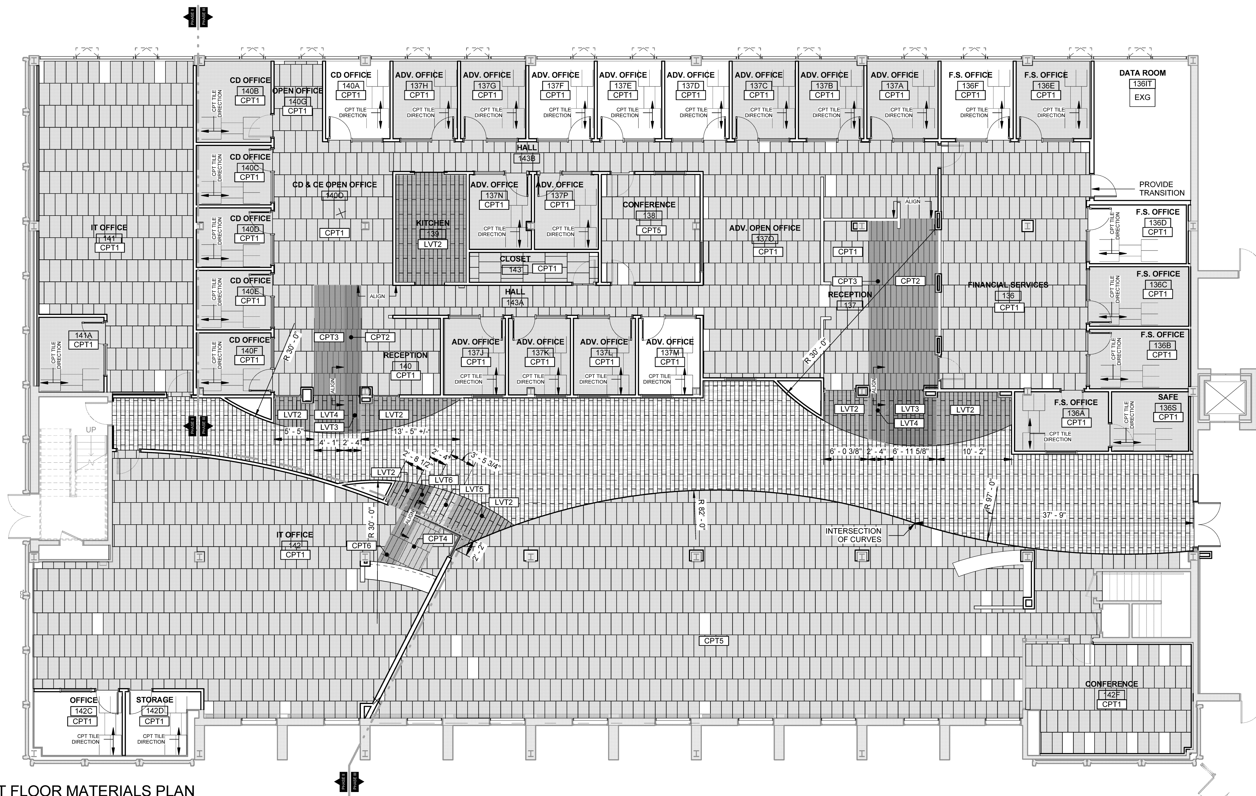
A1 FIRST FLOOR MATERIALS PLAN SCALE: 1/8" = 1'-0"
