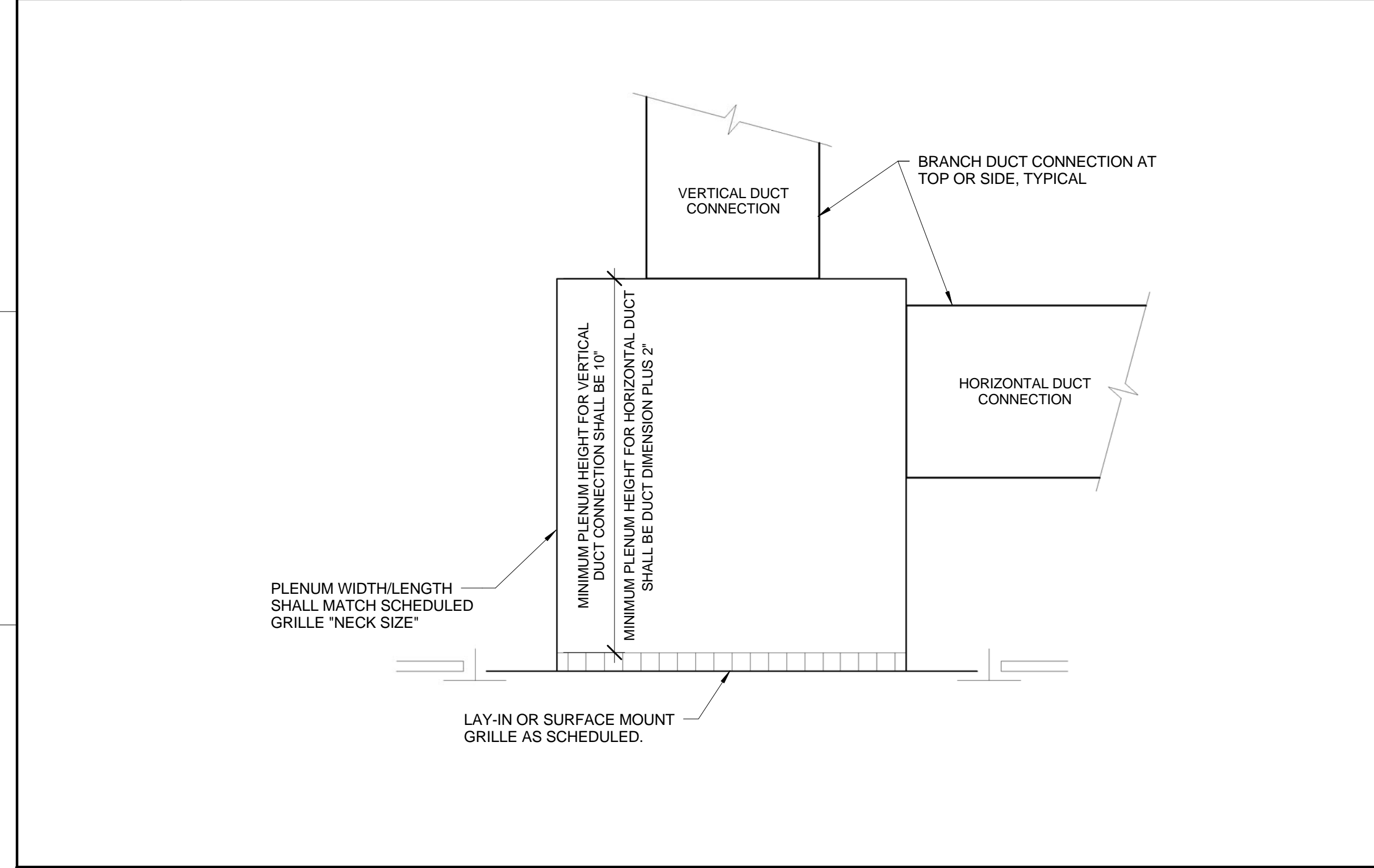
G1 DETAIL - RETURN AIR REGISTER BOOT NONE
