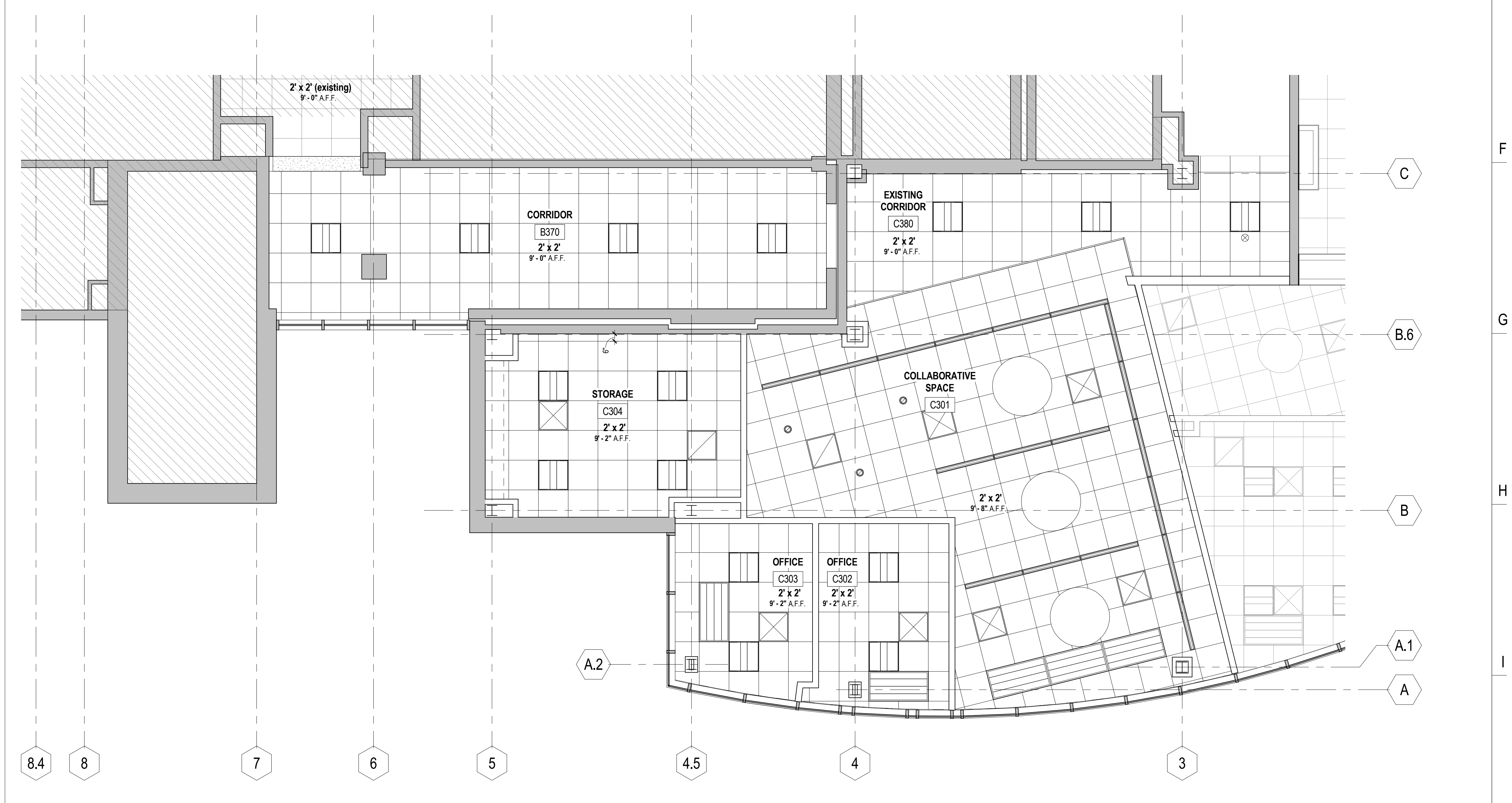
J5 LEVEL 3 - ALTERNATE NO. 1 A1.4 1/4" = 1'-0"
