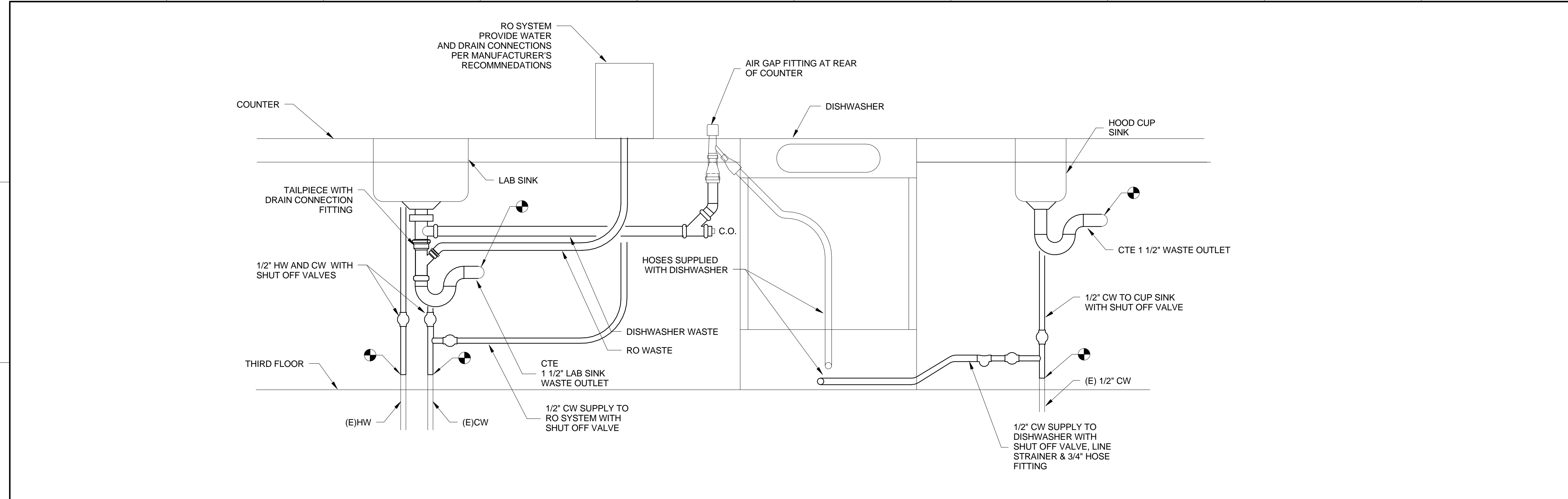
C1 DETAIL - PREP ROOM PLUMBING
