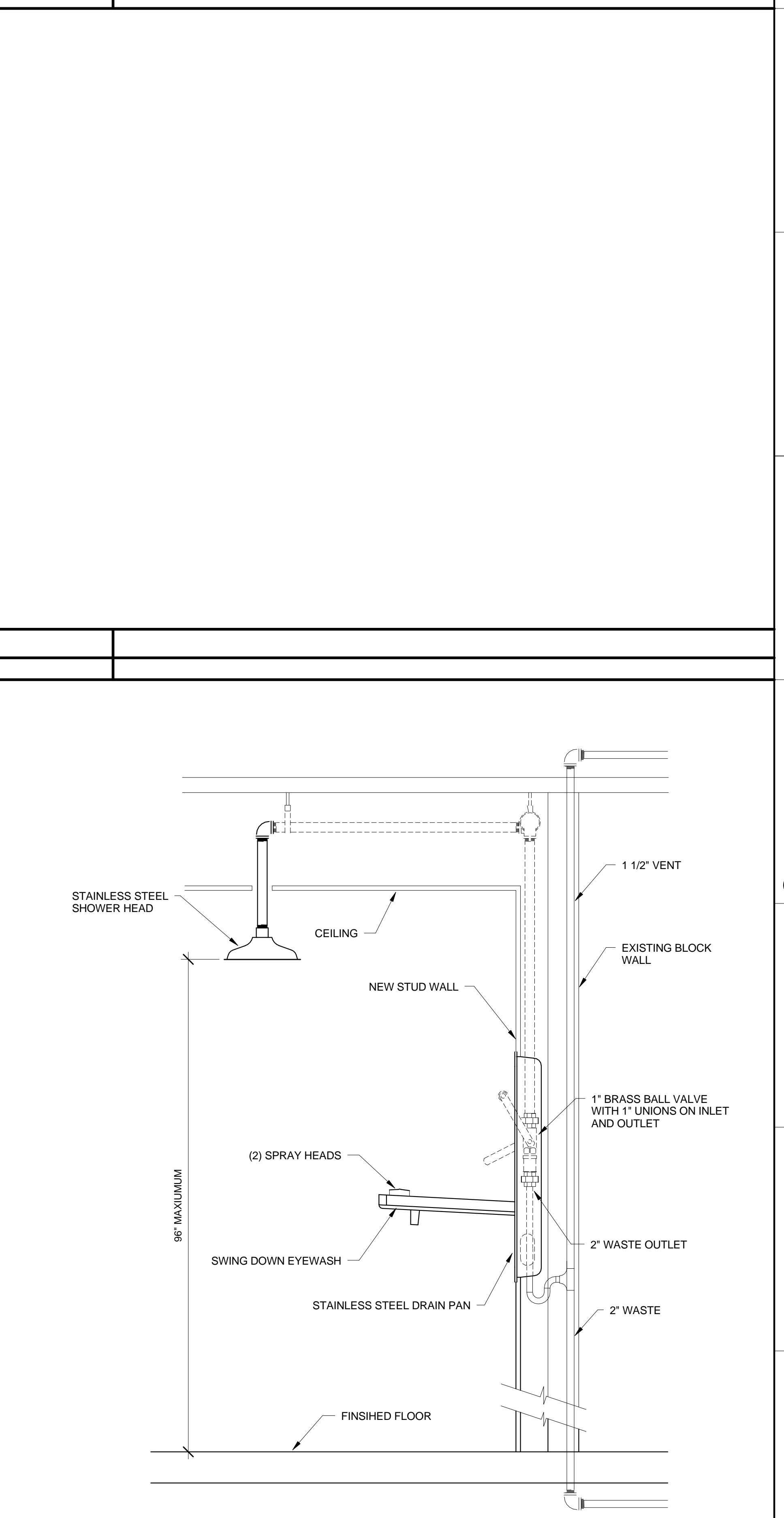
J11 DETAIL - SAFETY STATION SS-1
