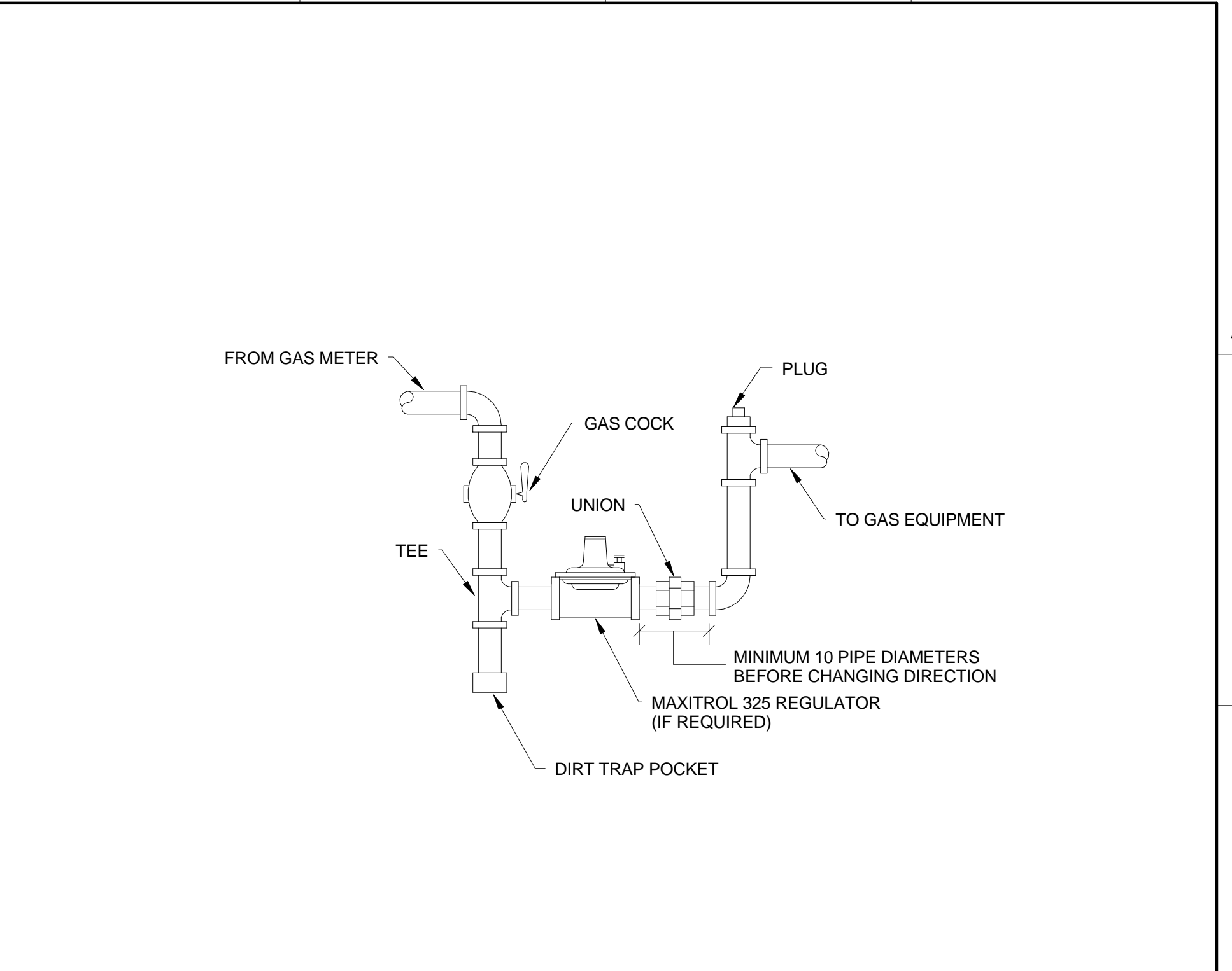
C11 DETAIL - GAS EQUIPMENT CONNECTION
