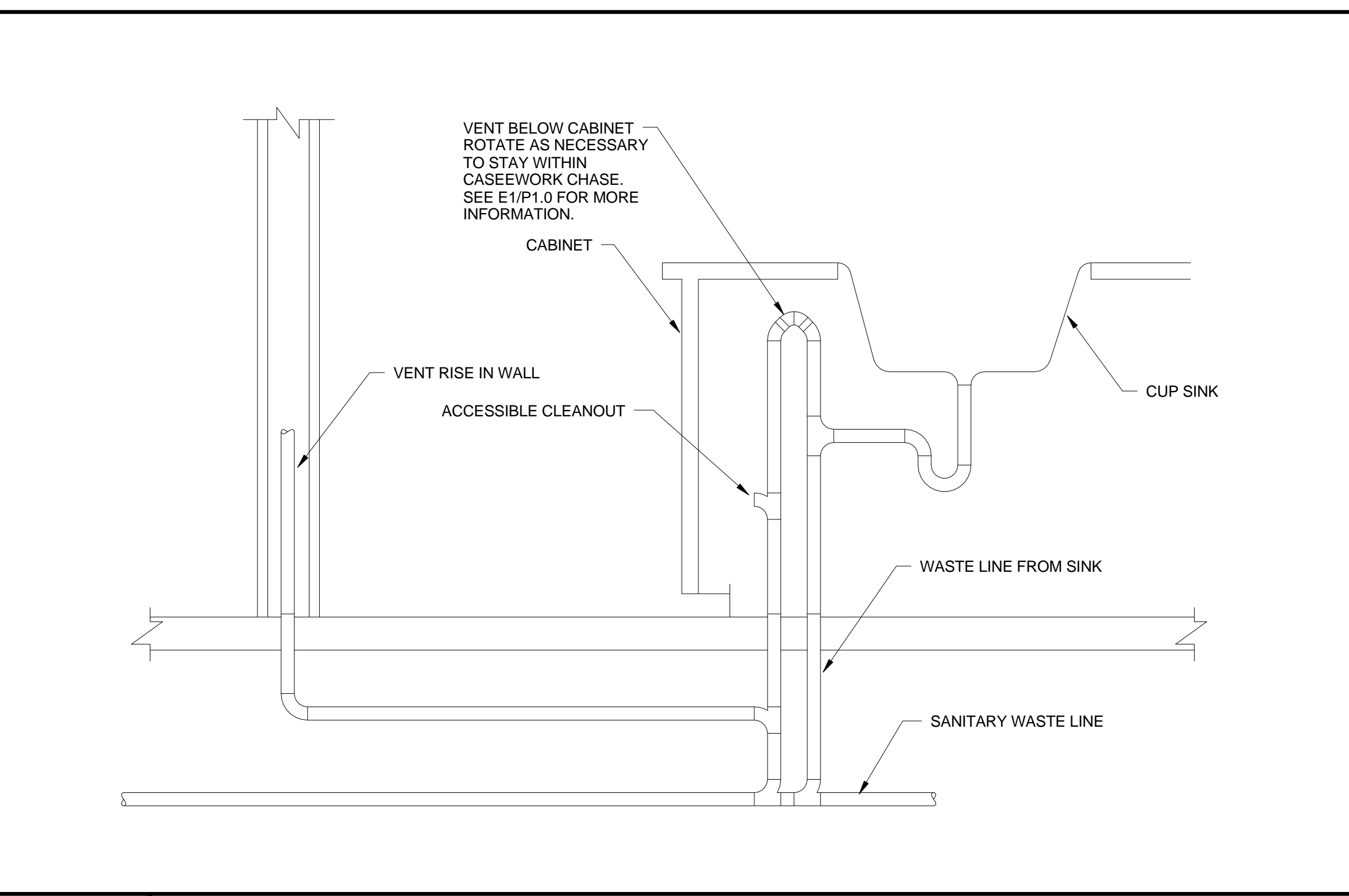
F6 DETAIL - ISLAND VENT
