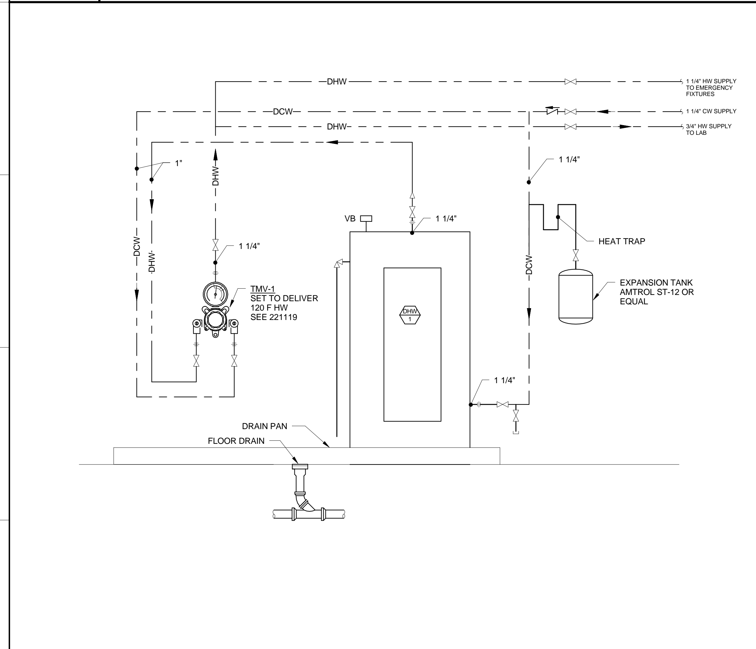
J1 DETAIL - ELECTRIC WATER HEATER
